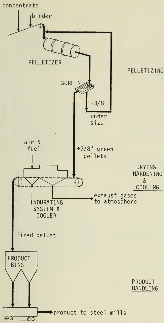
FIGURE 16 Agglomeration of iron ore concentrate
