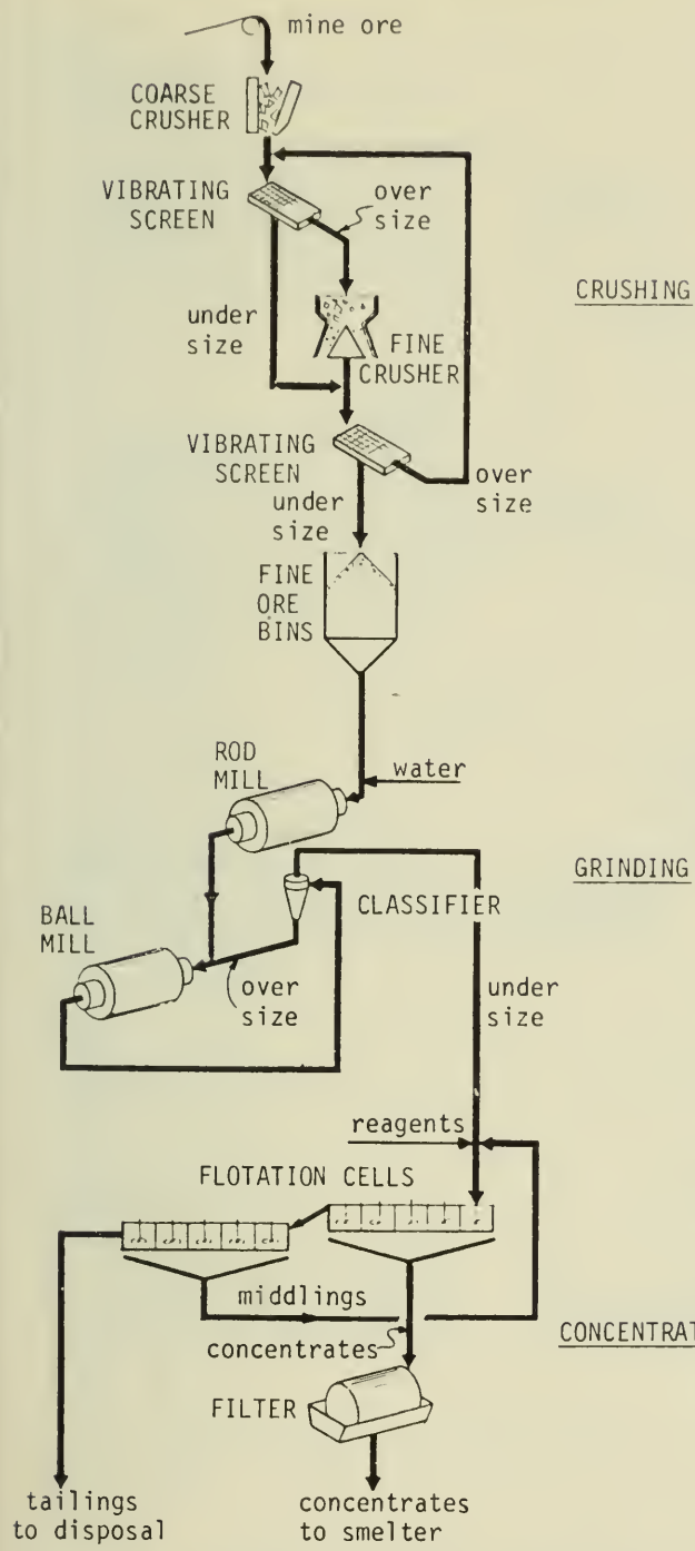
FIGURE 14 Crushing, grinding, and concentration
