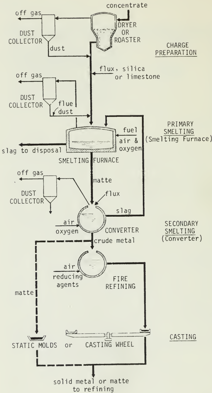
FIGURE 15 Smelting of concentrate
