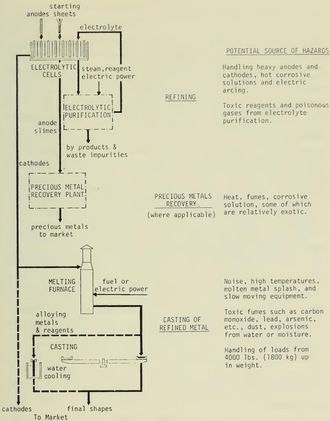
FIGURE 18 Electrolytic refining of metals
