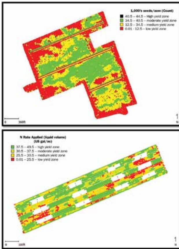
Figure 11-2. Screen captures comparing strips to blocks with nitrogen applied using variable rate technology.
