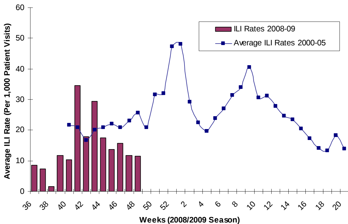
Figure 4: Average influenza-like illness (ILI) consultation rate (per 1,000 patient visits) reported by sentinel physicians* in Ontario in 2008- 2009 season, by report week, Compared to Ontario average † (1999/2000 to 2004/05 seasons).
