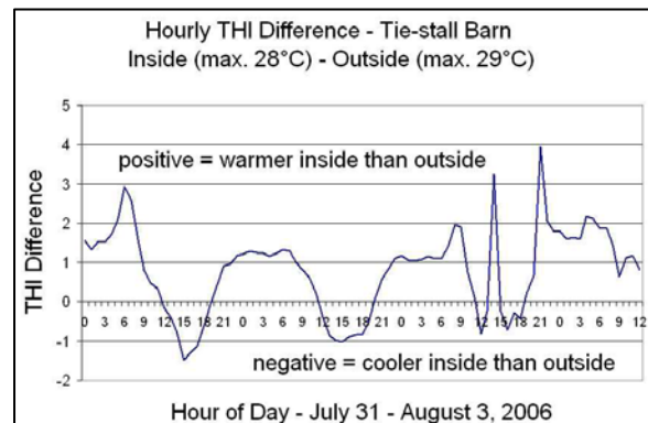
Figure 3. THI Difference – inside minus outside
