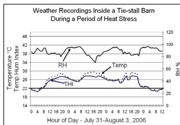
Figure 1. Inside Temperature, Temperature Humidity Index, Relative Humidity
