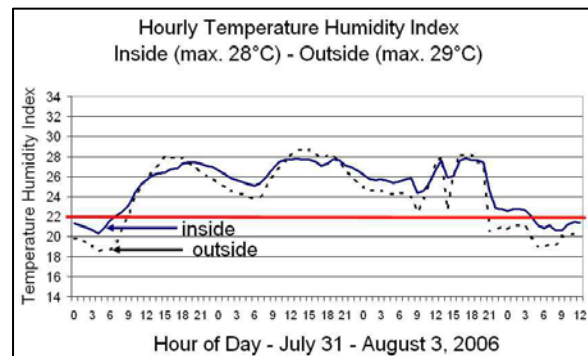
Figure 2. Hourly Temperature Humidity Index (THI)
