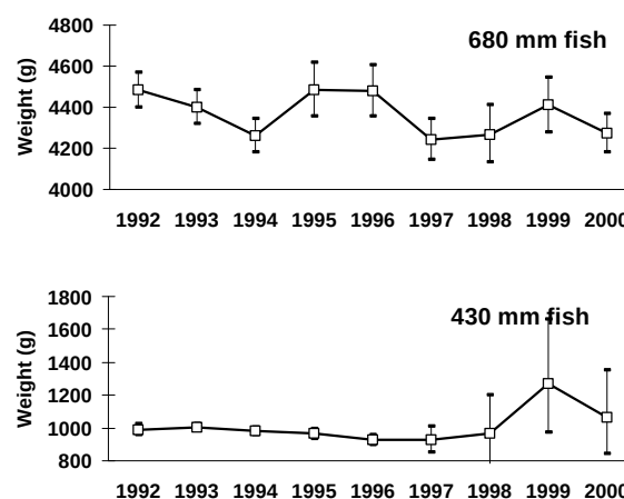
FIG. 4. Lake trout body condition, expressed as predicted weights of 430 and 680 mm fish. The weights were calculated from regression of log transformed round weight on log transformed fork length, and only data from 50 mm brackets around the shown values of fork length were used in the regressions (405-455 mm and 655-705 mm). The error bars represent 95% confidence intervals on the estimated weight.
