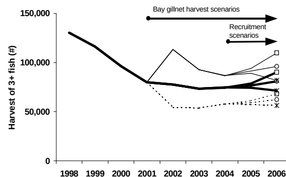
FIG. 7. Harvest of 3-year old and older fish predicted from simulations under various reproduction and exploitation scenarios. See Fig. 6 for interpretation.
