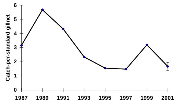
FIG. 4. Smallmouth bass catch in standard gillnets set in the Thousand Islands area, St. Lawrence River, 1987-2001. 95% confidence limits were not applied to corrected historical data.
