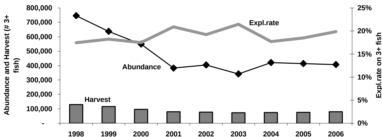
FIG. 4. Walleye population abundance, total harvest, and overall exploitation rate from simulation using best estimates of reproduction and exploitation levels (baseline scenario). All statistics are based on 3-years old and older fish.
