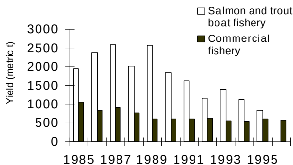
FIG. 4. Lakewide yields from Lake Ontario's New York and Ontario angling boat fishery for salmonids and from Ontario's commercial fishery, 1985-1996. The total boat-angling harvest was not measured in 1996.
