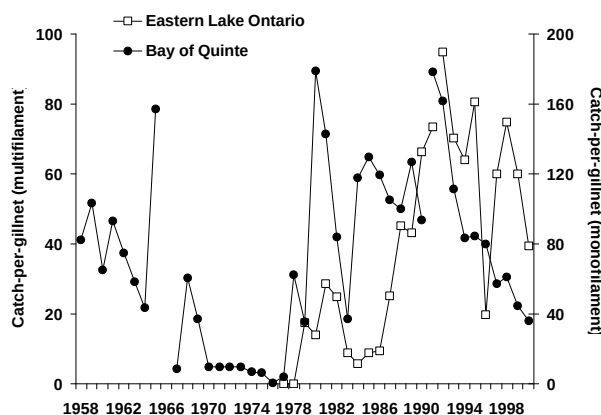
FIG. 2. Walleye abundance in gillnets in the Bay of Quinte, 1958-2000 (no gillnetting in 1966) and eastern Lake Ontario, 1977-2001, during summer. Multifilament gillnets were replaced with monofilament in 1991 in the Bay of Quinte and in 1992 in eastern Lake Ontario. The secondary y-axis is scaled by a factor of two relative to the primary y-axis because mono/multifilament gear comparisons showed that monofilament gillnets caught twice as many walleye.
