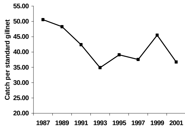
FIG. 1. Total number of fish captured in standard gillnets in the Thousand Islands area, St. Lawrence River, 1987-2001.
