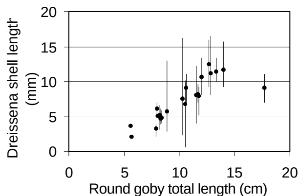
FIG. 3. Mean size and range of Dreissena found in the stomachs of the round gobies.
