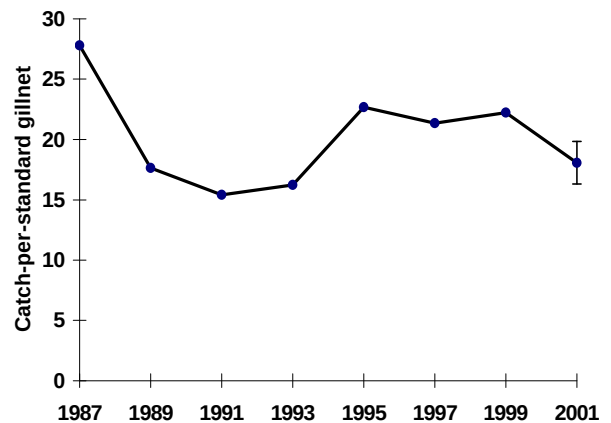
FIG. 3. Yellow perch catch in standard gillnets set in the Thousand Islands area 1987-2001. 95% confidence intervals were not applied to corrected historical data.
