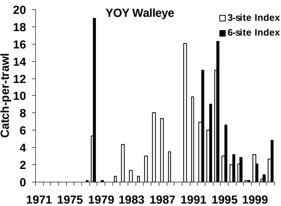
FIG. 12. Young-of-the-year walleye catch-per-trawl in the Bay of Quinte, 1972 to 2001 (no trawling in 1989) at 3 sites (Big Bay, Hay Bay and Conway), and 1972 to 1980, 1992 to 2001 (no trawling in 1989) at six sites (3 above plus Trenton, Belleville, and Deseronto).
