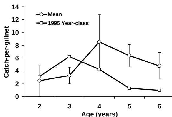
FIG. 5. Smallmouth bass catch-per-gillnet (Outlet Basin, Lake Ontario), at successive ages for the 1995 year-class and the mean ( \pm 2\text{SE} ) for four other strong year-classes (1980, 1983, 1987 and 1988) for comparison.
