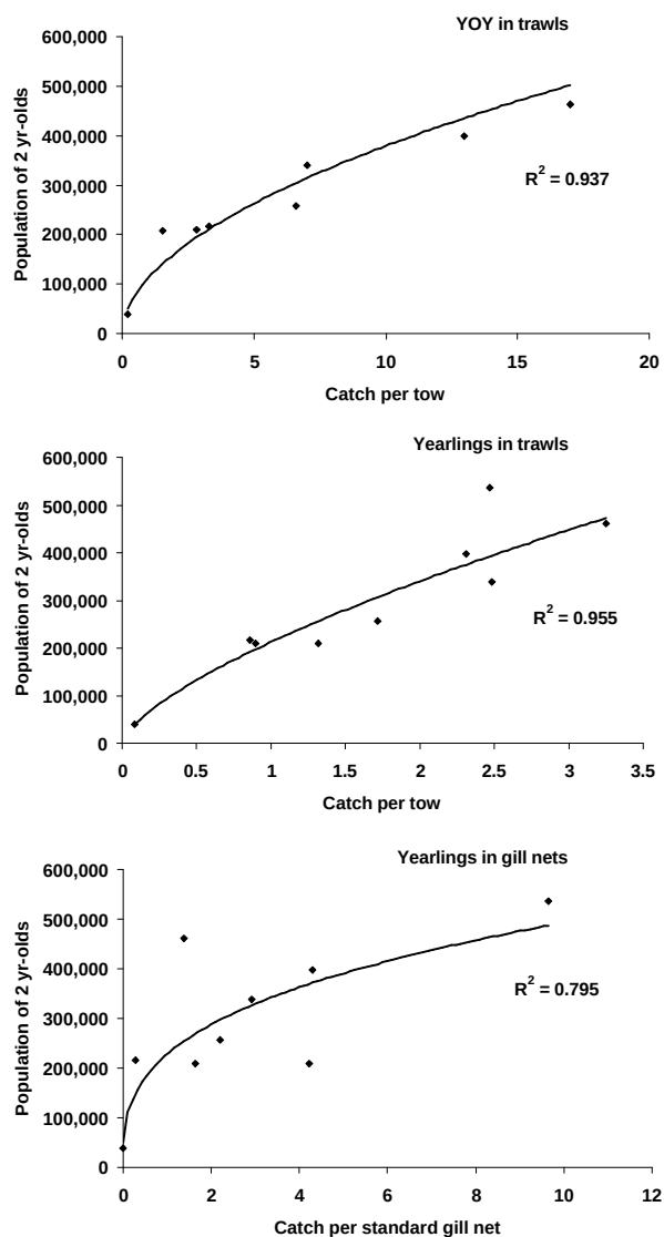
FIG. 9. The relationship between recruitment indices and population of 2 year-olds for the same year class of walleye in eastern Lake Ontario. The population estimate is for 1992-2001 using adjusted index netting estimates. The fit for a power function and its R^2 is indicated.
