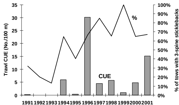
FIG. 5. Catches of threespine stickleback with mid-water trawl in summer surveys. Bars represent yearly catch per unit effort; line shows proportion of tows that contained sticklebacks.
