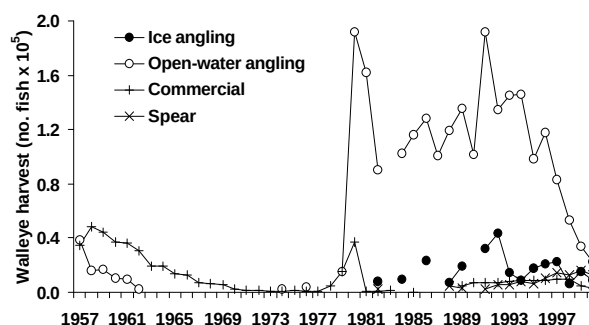
FIG. 4. Trends in walleye harvest by open-water angling (1957-1962, 1976, and 1979-2000), ice-angling (1982, 1984, 1986, 1988, 1989, and 1991-2001), commercial (1957-2000), and aboriginal spear fisheries (1982, 1988 and 1989, and 1991-2000).
