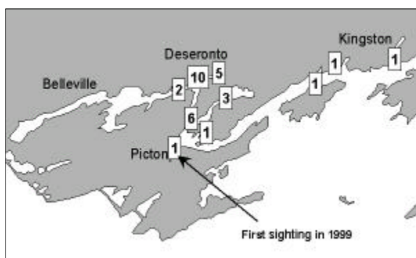
FIG. 13. Sightings of round gobies in Eastern Lake Ontario in 2001. Numbers of angler reports are shown; each report may contain more than one goby.
