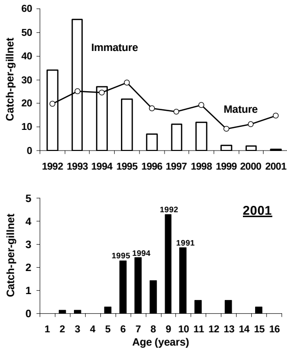
FIG. 8. Lake whitefish catch-per-gillnet for immature (open bars) and mature (line) fish in the Outlet Basin of Lake Ontario, 1992 to 2001 (top panel), and lake whitefish age distribution in 2001 (lower panel). Strong year-classes are indicated.
