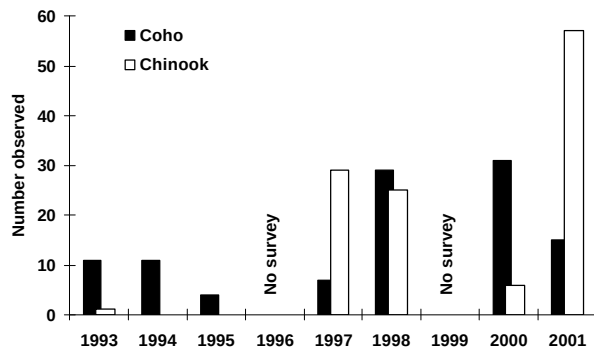
FIG. 10. Number of YOY coho and chinook salmon observed during summer surveys of Lake Ontario tributaries in Ontario. No surveys were conducted in 1996 and 1999.
