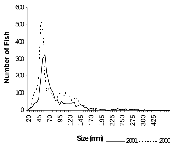
Fig. 2. Plot illustrating the size distribution of all fish caught in both the 2000 and 2001 trawls.
