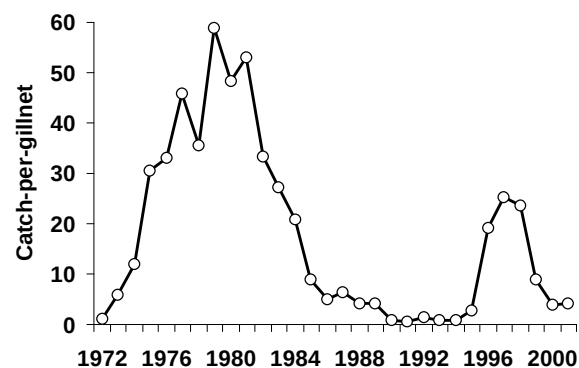
FIG. 6. Smallmouth bass abundance (3-yr running average) in Bay of Quinte index gillnets (Big Bay site) during mid-summer, 1972 to 2001.
