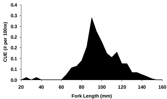
FIG. 3. Length frequency distribution of rainbow smelt in mid-water trawls conducted in August 2001.
