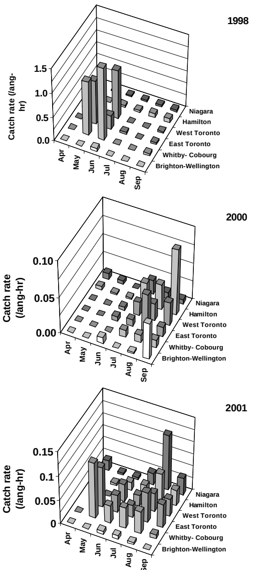
FIG. 11. The seasonal and spatial pattern of catch rates of rainbow trout by launch daily anglers in western Lake Ontario during 1998, 2000, and 2001.
