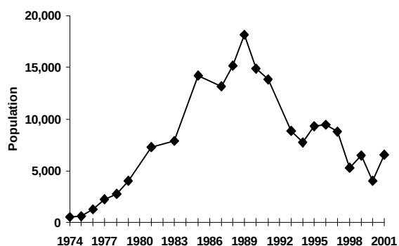
FIG. 12. The estimated upstream count of rainbow trout at the Ganaraska River fishway at Port Hope, Ontario during April and May.
