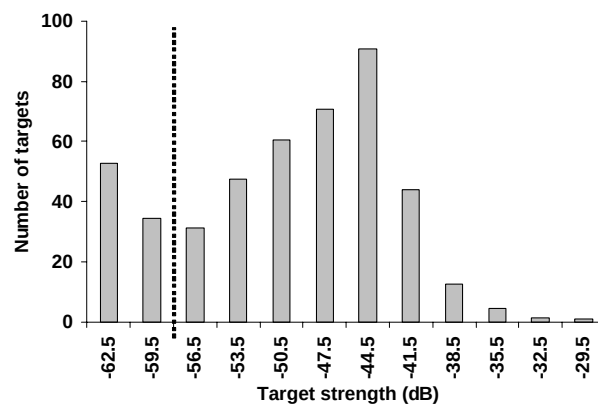
FIG. 3. Acoustic target strength distribution from the hypolimnion (data from summer 2000 shown here as a representative example). Targets larger than -58dB
