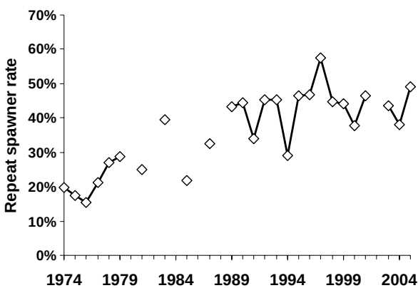
FIG. 2.1.2. The repeat spawner rate for rainbow trout (sexes combined) in April at the Ganaraska River fishway, in Port Hope, Ontario, 1974-2005.
