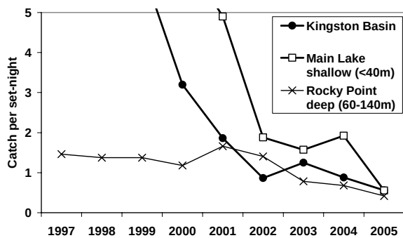
FIG. 2.3.3. Catch per unit effort of adult lake trout in bottom-set gillnets in three areas of eastern lake Ontario.
