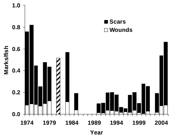
FIG. 2.1.3. Lamprey mark trends on rainbow trout in April, 1974-2005, at the Ganaraska River fishway in Port Hope, Ontario. Since 1990, A1 and A2 marks 1 were called wounds and the remainder of marks were called scars to fit with historical classification. Scars and wounds were combined in 1981.
