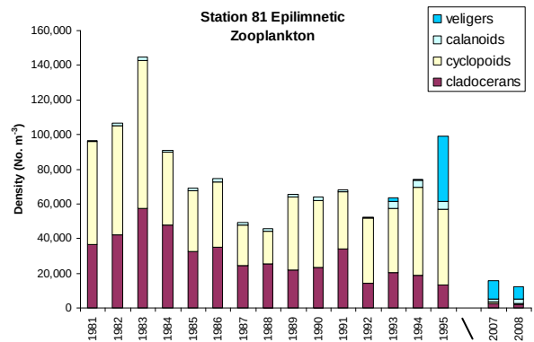
Fig. 9.3.1. Seasonal mean density (No·m -3 ) of dominant zooplankton groups in the epilimnion at Station 81 from 1981-95 and 2007-08.
