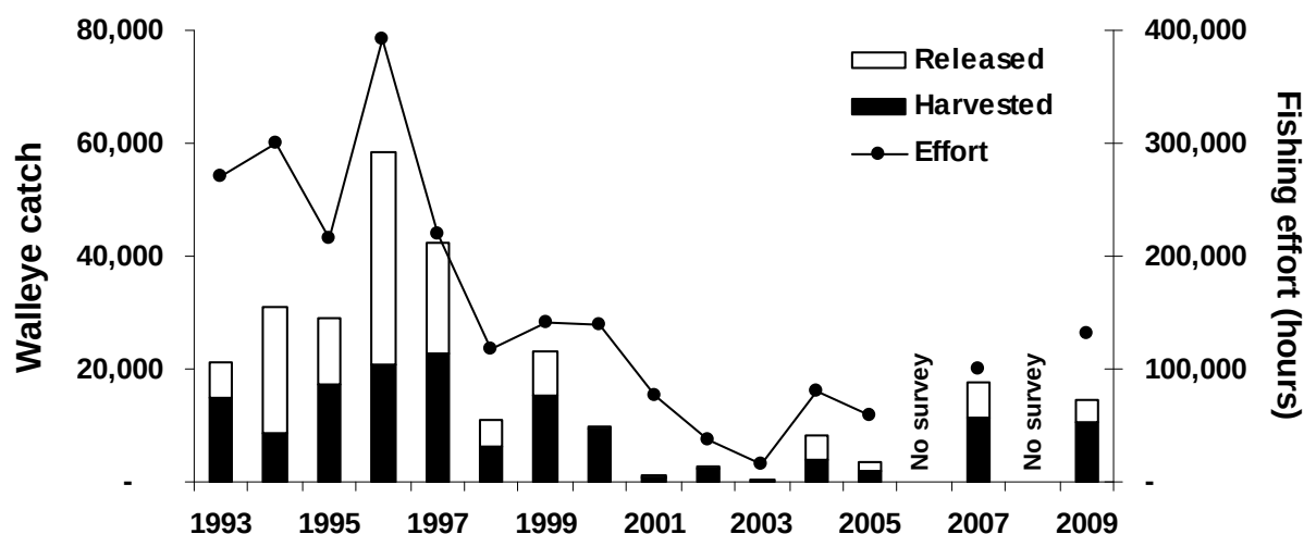
FIG. 3.1.1. Fishing effort and walleye catch (released and harvested) during the winter ice-fishery, 1993-2009. No data for 2006 or 2008.
