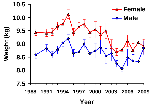
FIG. 2.9.1. Mean weight (+ 95%) of a 900 mm Chinook salmon in the Credit River, 1989-2009, during the spawning run (approximately Oct 1 each year).
