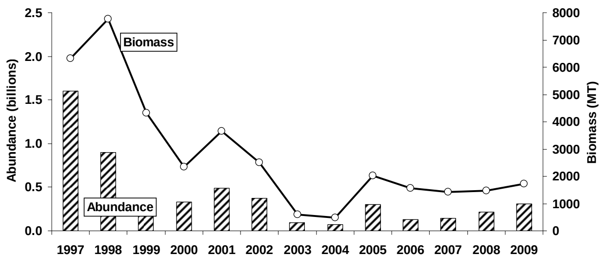
FIG. 2.5.2. Abundance and biomass of yearling-and-older rainbow smelt . Abundance estimates were obtained directly from hydroacoustic surveys, biomass estimates were obtained by applying average weights to abundance estimates. The weight information normally comes from midwater trawls done during the surveys, however information from other sources was used for years 2002, 2004, 2005, 2008 and 2009.
