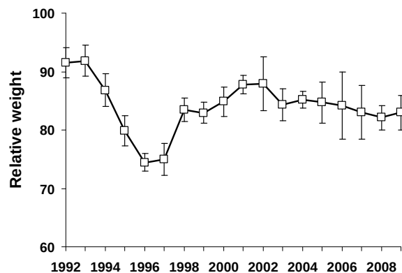
FIG. 2.3.3. Lake whitefish relative weight (see 1 Rennie et al. 2008) for fish caught in summer index gillnets, 1992-2009.
