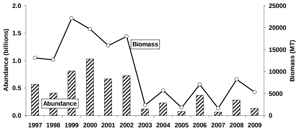
FIG. 2.5.1. Abundance and biomass of yearling-and-older alewife . Abundance estimates were obtained directly from hydroacoustic surveys, biomass estimates were obtained by applying average weights to abundance estimates. The weight information normally comes from midwater trawls done during the surveys, however information from other sources was used for years 2002, 2004, 2005, 2008 and 2009.
