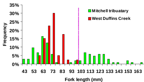
FIG. 2.8.3. Fork length distribution of Atlantic salmon in Duffins Creek in 2009. The dotted line indicates the 100 mm division, above which Atlantic salmon are expected to smolt in 2010.
