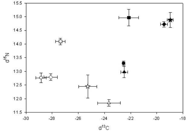
FIG. 8.4.1. Mean \pm standard error \delta^{13}\text{C} and \delta^{15}\text{N} measurements for fish from warm (Upper Bay, open symbols) and cool (Lower Bay, solid symbols) environments in the Bay of Quinte, Lake Ontario. Species include: alewife (circles), round goby (triangles), yellow perch (diamonds), largemouth bass (stars), and walleye (squares).
