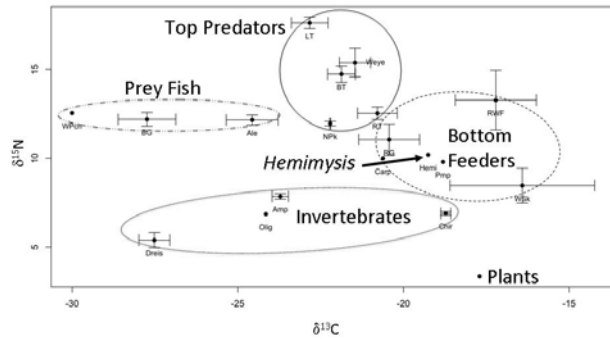
FIG. 8.2.1. Food web structure at Cobourg, Lake Ontario in fall 2009 as revealed by stable isotopes of ^{13}\text{C} and ^{15}\text{N} . Results are preliminary, with additional taxa undergoing analyses.
