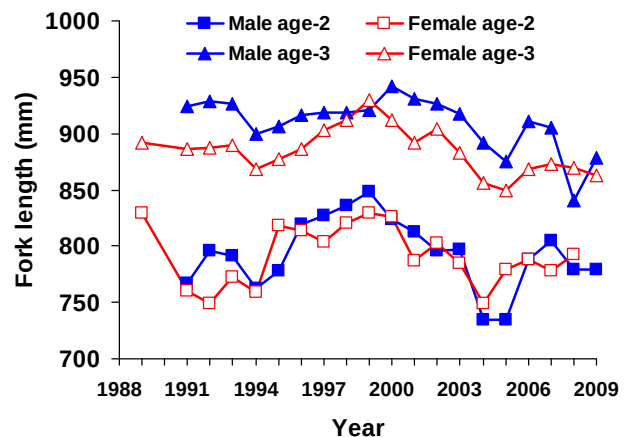
FIG. 2.9.2. Fork length by sex of age-2 and age-3 mature Chinook salmon in the Credit River, 1989-2009, during the spawning run (approximately Oct 1 each year).
