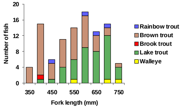
FIG. 2.2.2. Fork length of salmon, trout, and walleye observed in gillnets in central Lake Ontario, during May 2009.
