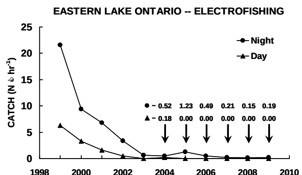
FIG. 7.3.4. Electrofishing catch of American eel (numbers caught per hr) in eastern Lake Ontario, separated by day and night for a recent period of 1999-2009.
