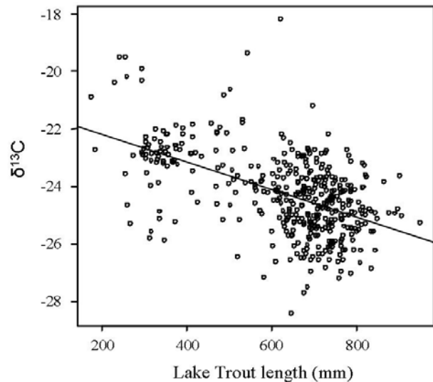
FIG. 8.3.1. Relationship between fish size and muscle \delta^{13}\text{C} in Lake Ontario lake trout, 2008.
