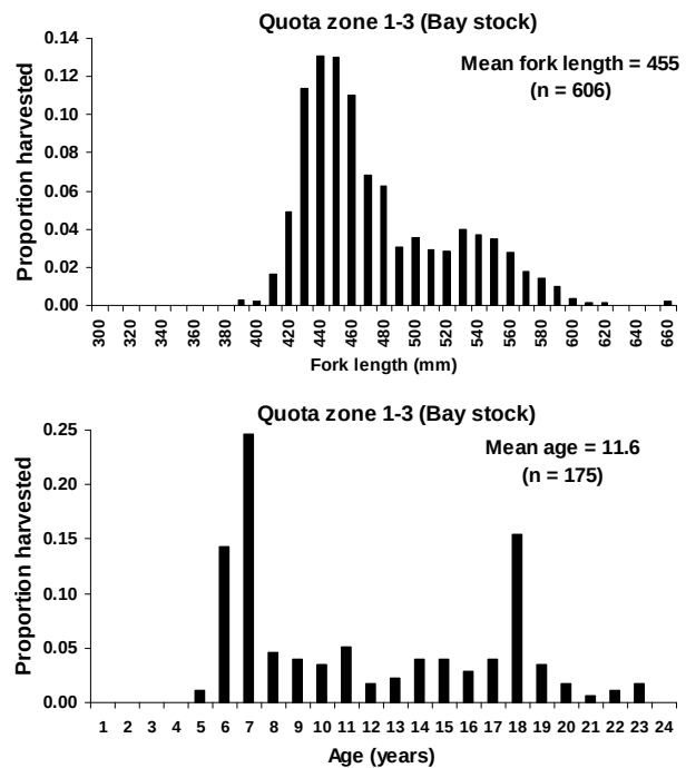
FIG. 4.2.2. Size and age distribution (by number) of lake whitefish sampled in QZ 1-3 during the 2009 commercial catch sampling program.
