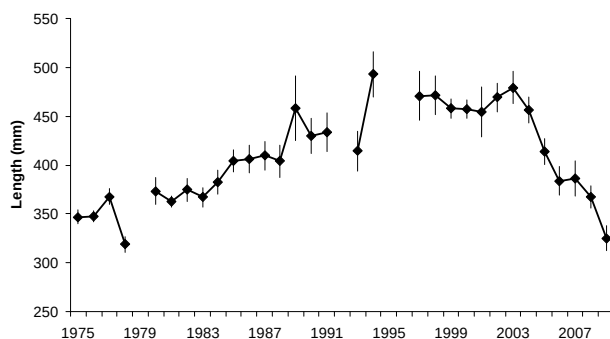
FIG. 7.3.3. Length (error bars are 95% confidence limits) of eel migrating upstream through the eel ladder located at the R.H. Saunders Hydroelectric Dam, 1975-2009.
