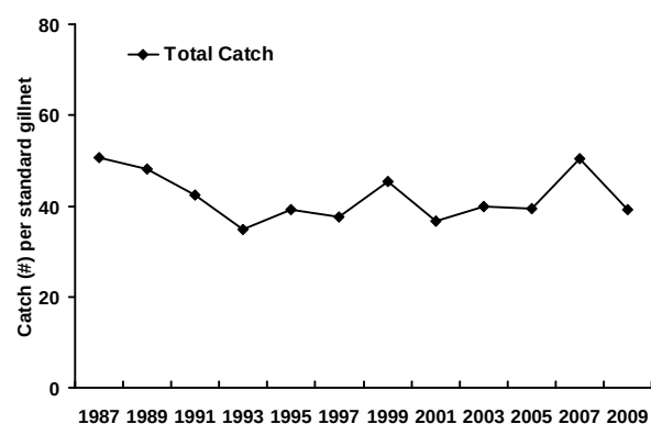
FIG. 2.7.1. Total number of fish (all species) per standard gillnet set in the Thousand Islands area of the St. Lawrence River, 1987-2009.
