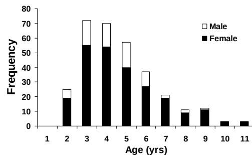
FIG. 4.3.1. Age distribution, by sex, of commercially harvested northern pike sampled during the 2009 Observer program.
