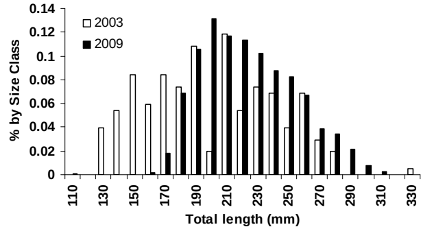
FIG. 3.2.2. Size distribution of angler caught yellow perch sampled in the 2003 and 2009 recreational angler surveys.
