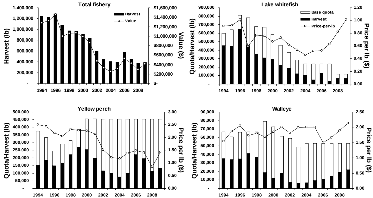
FIG. 4.1.2. Total harvest and value for the Lake Ontario commercial fishery and quota, harvest and price-per-lb for lake whitefish, yellow perch and walleye, 1994-2009.
