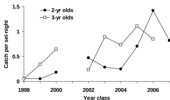
FIG. 2.3.6. Relative survival of lake trout to ages 2 and 3. The survival index is the catch per unit effort of 2 and 3 year old fish, corrected for number stocked 2 or 3 years earlier; age determination is based on of year-specific fin clip information combined with the size of the fish.
