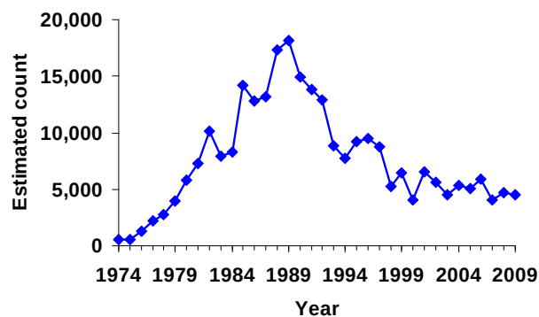
FIG. 2.1.1. Estimated upstream counts of rainbow trout at the Ganaraska River fishway, Port Hope, Ontario during April and May, 1974-2009. Estimates for 1980, 1982, 1984, 1986, 1992, and 2002 were interpolated from adjacent years.
