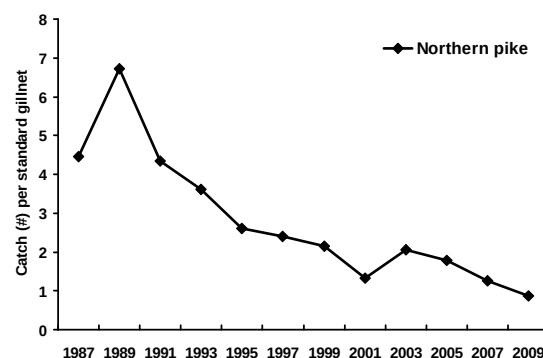
FIG. 2.7.6. Northern pike catch per standard gillnet set in the Thousand Islands area of the St. Lawrence River, 1987-2009.
