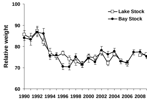
FIG. 4.2.3. Lake whitefish (Lake Ontario and Bay of Quinte spawning stocks and sexes combined) relative weight (see Rennie et al. 2008), 1990-2009.
