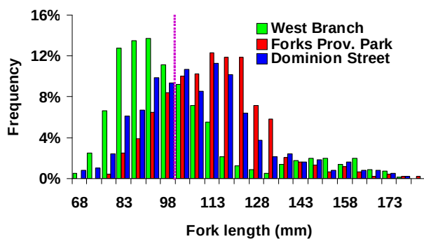
FIG. 2.8.4. Fork length distribution of Atlantic salmon in the Credit River in 2009. The dotted line indicates the 100 mm division, above which Atlantic salmon are expected to smolt in 2010.
