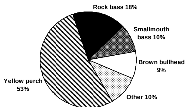
FIG. 2.7.2. Species composition in the 2009 gillnet survey in the Thousand Island area of the St. Lawrence River.
