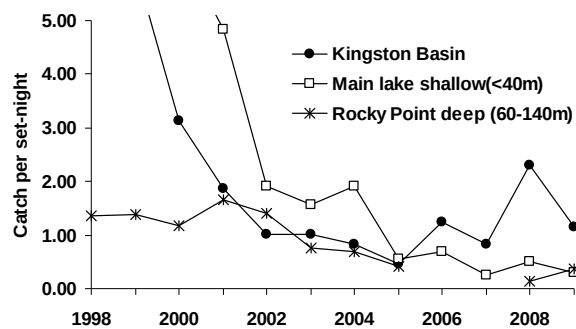
FIG. 2.3.4. Catch per unit effort of adult lake trout in bottom-set gillnets in three areas of eastern lake Ontario. Deep sets off Rocky Point were not fished in 2006 and 2007.
