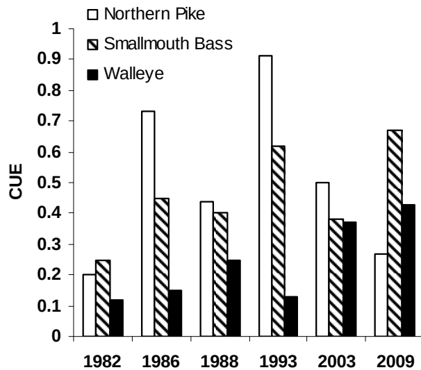
FIG. 3.2.1. Catch per-unit effort values compared for popular species on Lake St. Francis (except yellow perch) for the years 1982, 1986, 1988, 1993, 2003, and 2009.
