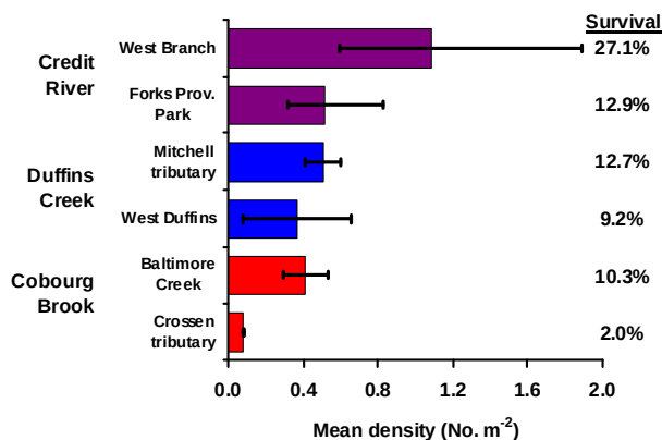
FIG. 2.8.1. Mean density and survival of young-of-the-year Atlantic salmon in the Credit River, Duffins Creek, and Cobourg Brook at sites stocked with a density 4 spring fingerlings m -2 in 2009. Error bars indicate the 95% confidence interval of mean density.
