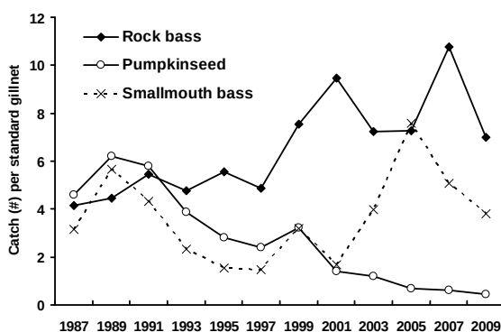
FIG. 2.7.4. Centrarchid catches per standard gillnet set in the Thousand Islands area of the St. Lawrence River, 1987-2009.
