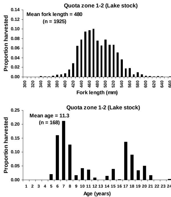
FIG. 4.2.1. Size and age distribution (by number) of lake whitefish sampled in QZ 1-2 during the 2009 commercial catch sampling program.
