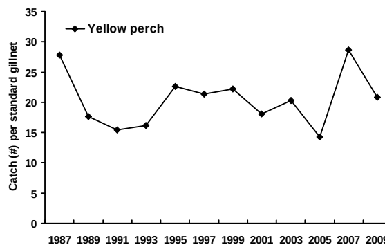
FIG. 2.7.3. Yellow perch catch per standard gillnet set in the Thousand Islands area of the St. Lawrence River, 1987-2009.
