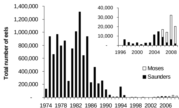
FIG. 7.3.2. Total number of eels ascending the eel ladder(s) at the Moses-Saunders Dam, Cornwall, Ontario for 1974-2009. No counts are available for 1996.
