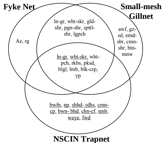
FIG. 8.5.1. All species captured in fyke nets, small-mesh gillnets, and NSCIN trapnets at eight sites in the Bay of Quinte, Lake Ontario, in the summer of 2009. Circles represent each type of net; species captured in more than one type of net are indicated in the appropriate over-lapping portion of the circles. Species names that are underlined were not small-bodied fish (i.e., they were > 20 cm in length). Ae=American eel, rg=round goby, ln-gr=longnose gar, wht-skr=white sucker, gld-shr=golden shiner, pgn-shr=pugnose shiner, spttl-shr=spottail shiner, lgpch=logperch, awf=alewife, gzsd=gizzard shad, emd-shr=emerald shiner, cmn-shr=common shiner, btn-mnw=bluntnose minnow, wht-pch=white perch, rkbs=rockbass, pkds=pumpkinseed, blgl=bluegill, lmb=largemouth bass, blk-crp=black crappie, yp=yellow perch, bwn=bowfin, np=northern pike, shhd-rdhs=shorthead redhorse, cmn-cp=common carp, bwn-bhd=brown bullhead, chn-cf=channel catfish, smb=smallmouth bass, weye=walleye, fwd=freshwater drum.
