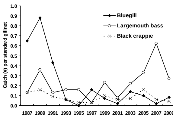
FIG. 2.7.5. Centrarchid catches per standard gillnet set in the Thousand Islands area of the St. Lawrence River, 1987-2009.
