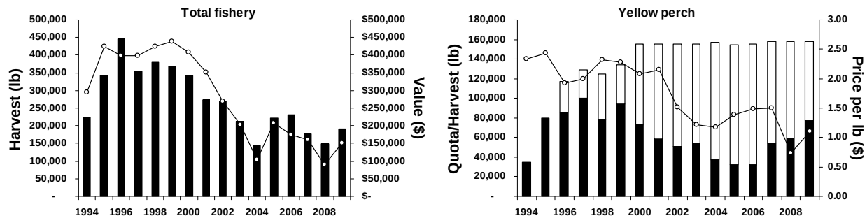
FIG. 4.1.3. Total harvest and value for the St. Lawrence River commercial fishery and quota, harvest and price-per-lb for yellow perch, 1994-2009.
