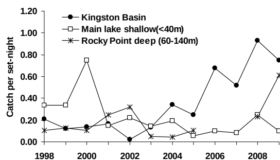
FIG. 2.3.5. Catch per unit effort of immature lake trout in bottom-set gillnets in three areas of eastern lake Ontario. Deep sets off Rocky Point were not fished in 2006 and 2007.
