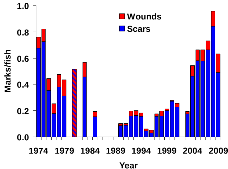
FIG. 2.1.2. Lamprey mark trends on rainbow trout in April, 1974-2009, at the Ganaraska River fishway, in Port Hope, Ontario. Since 1990, A1 and A2 marks were called wounds and the remainder of marks were called scars to fit with historical classification. Scars and wounds were combined in 1981.
