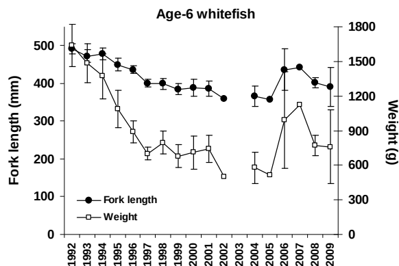
FIG. 2.3.2. Lake whitefish fork length and weight of an age-6 fish caught in summer index gillnets, 1992-2009. No age-6 fish was caught in 2003.
