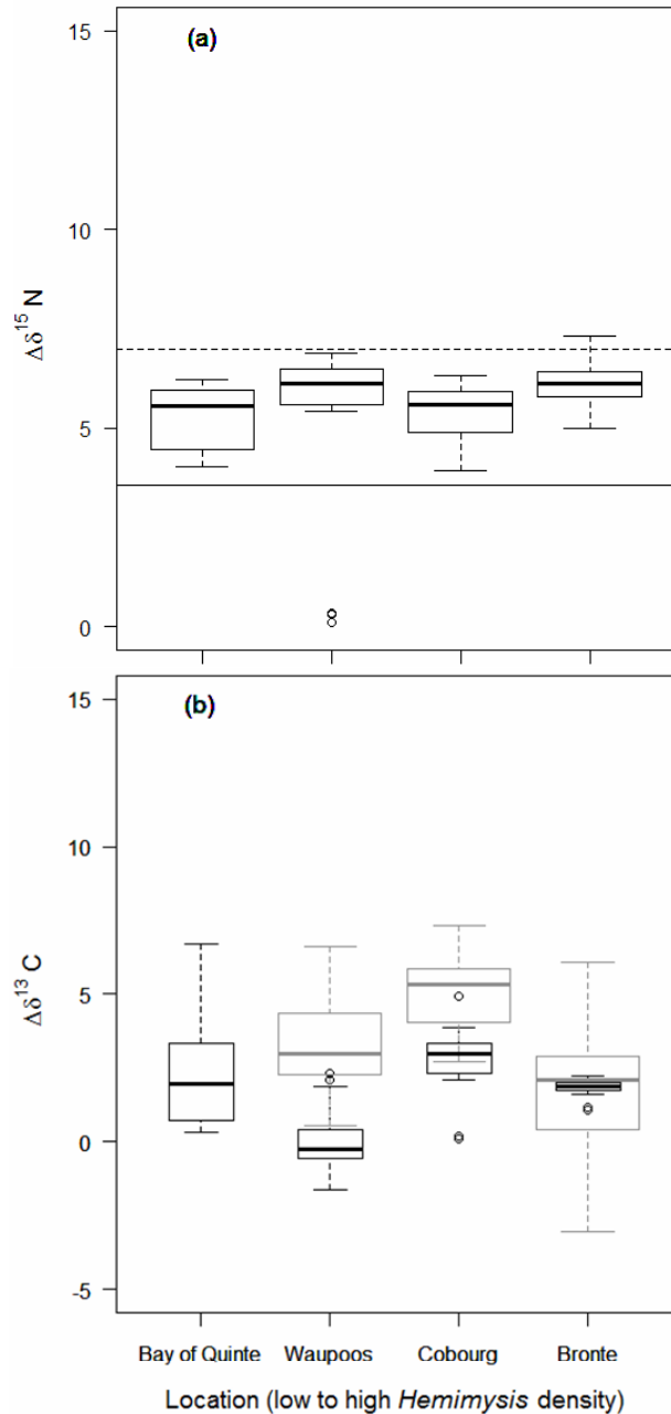
Fig. 10.1.1. \Delta\delta^{15}N and \Delta\delta^{13}C of alewife ( Alosa pseudoharengus ) (a and b, respectively) relative to the \Delta\delta^{15}N and \Delta\delta^{13}C of Hemimysis anomala (solid line and grey boxplots, respectively). The dashed line in (a) represents a 3.4 ‰ ^{15}N trophic enrichment of Hemimysis . Boxes in (a) that are close to the dashed lines indicate alewife are consuming prey similar to Hemimysis . Black boxes in (b) that overlap the grey boxes indicate alewife are consuming prey similar to Hemimysis . Combining (a) and (b) suggests alewife from Bronte are consuming Hemimysis .
