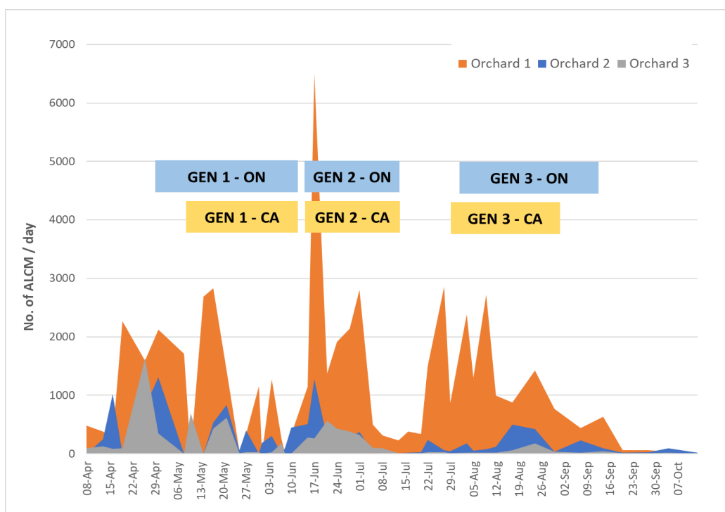
Figure 55. Number of apple leafcurling midge adult males trapped per day from 3 orchards in Norfolk County, ON from April to October 2021. Blue and yellow boxes represent predicted period of activity for first, second and third generations based on a regional degree day model for Ontario (Gen 1 – ON, Gen 2 – ON, Gen 3 – ON) and a national degree day model (Gen 1 – CA, Gen 2 – CA, Gen 3 – CA), respectively.
