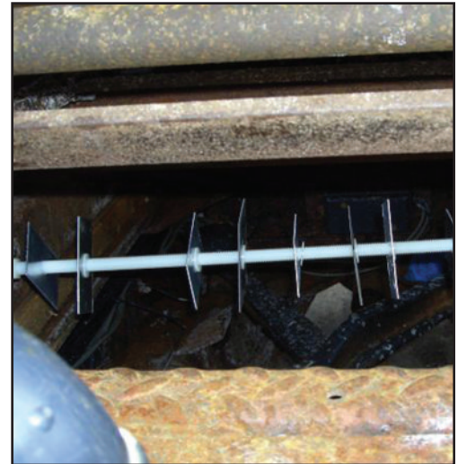
Metal coupons affixed to a winter maintenance vehicle test the effectiveness of corrosion inhibitors.
