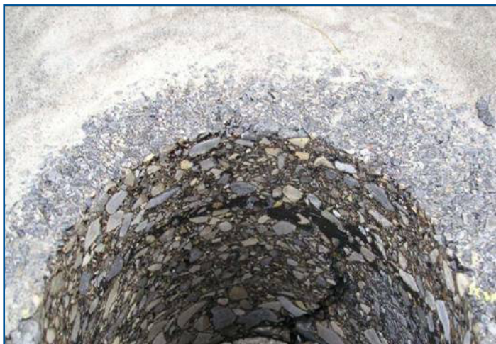
No visible crack propagation in core hole of section after using fibre-reinforced interlayer.
