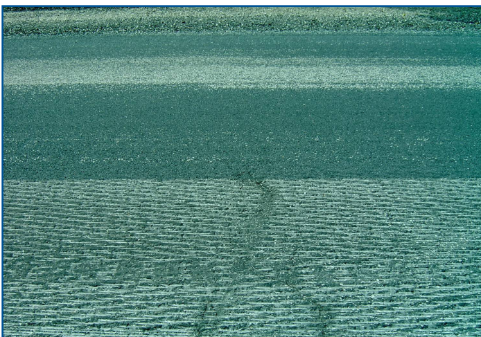
Example of Fibermat type B applied as a SAMI over a milled surface and awaiting a hot mix cap. Note the severity of the cracking to be inhibited by this interlayer.
