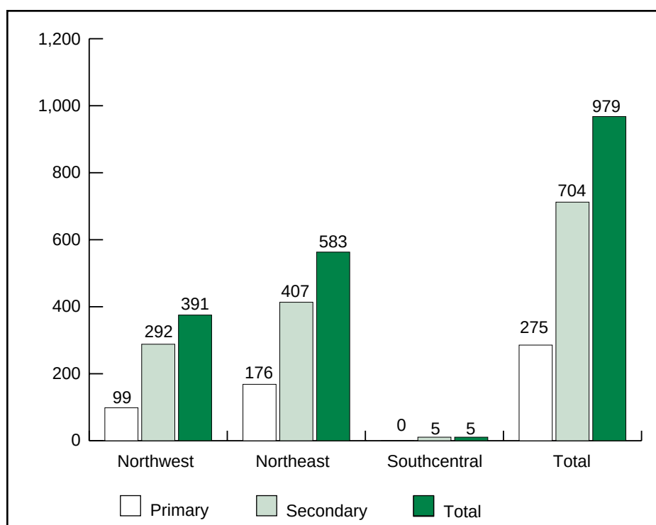
Figure 21 Road Construction (kilometres) 1997/98 by Road Class and MNR Region
