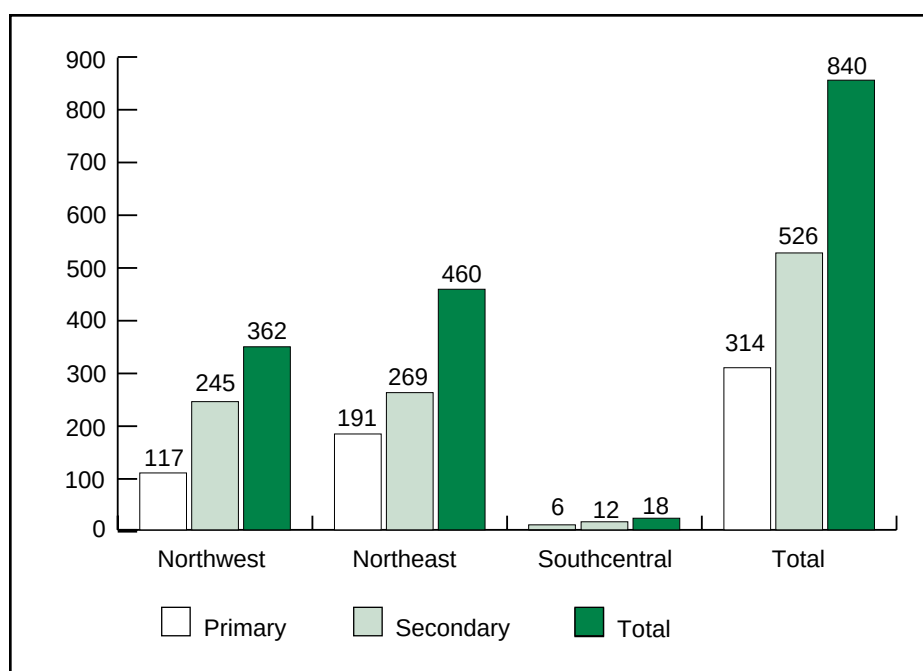
Figure 14 Road Construction (kilometres) in 1998/99 by Road Class and MNR Region
