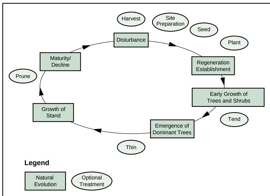
Figure 3 The Forest Life Cycle
