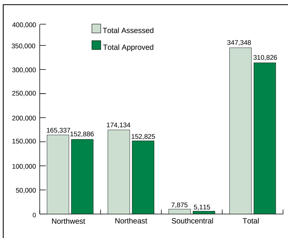
Figure 18 Summary of Area (hectares) Declared Free-To-Grow by MNR Region (1998/99)
