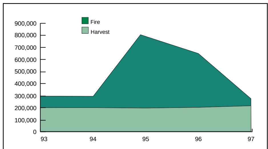
Figure 5 Forest Area (hectares) Disturbed by Harvest and Fire for all Crown Land (1993-1997)
