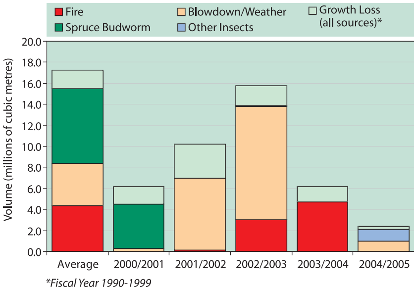
Figure 1 Summary of mortality and growth loss in the AOU.
