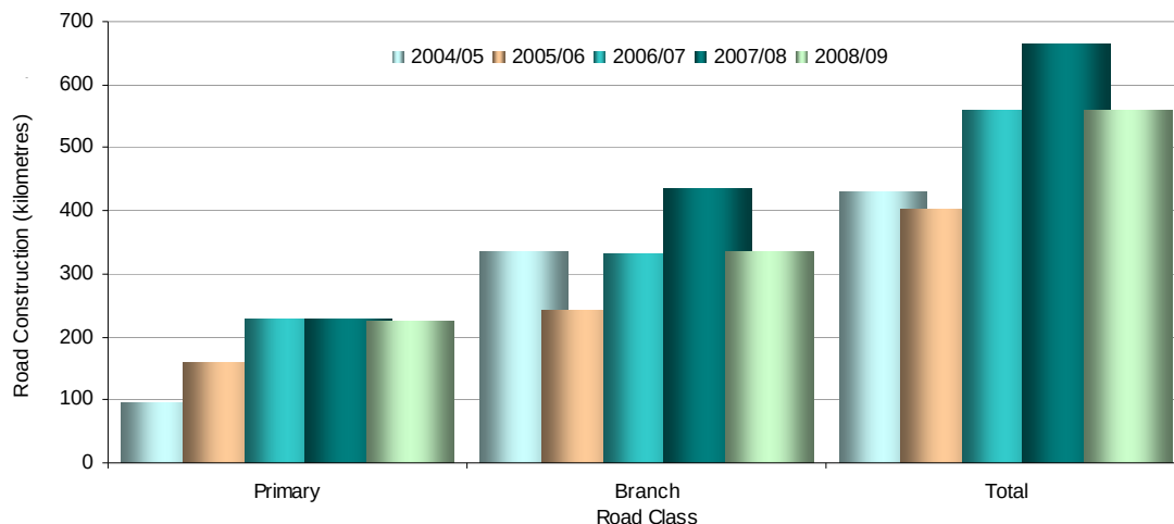
Figure 6a - Primary and branch road construction
