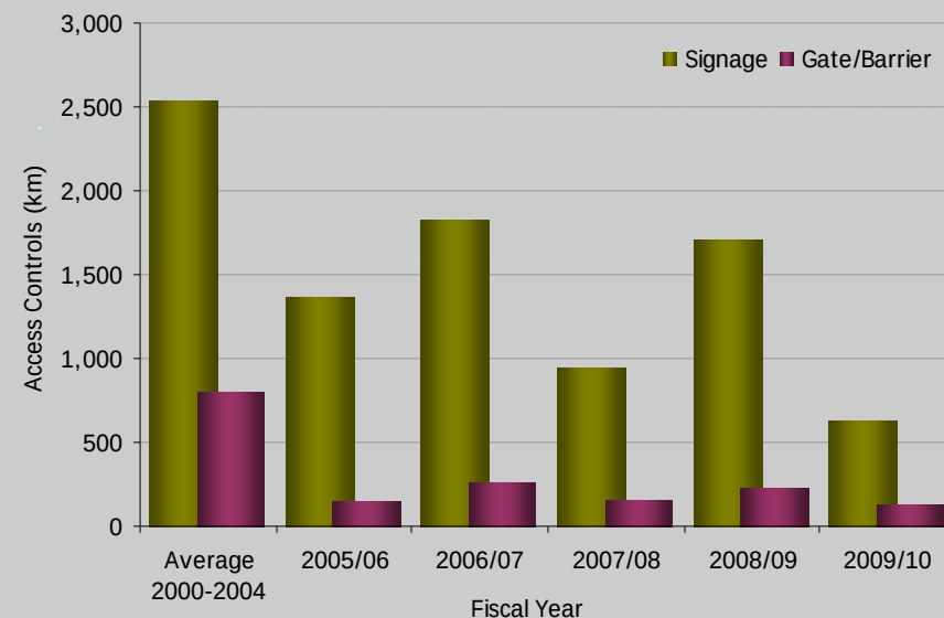
Figure 8c - Road Access Controls Established by Year
