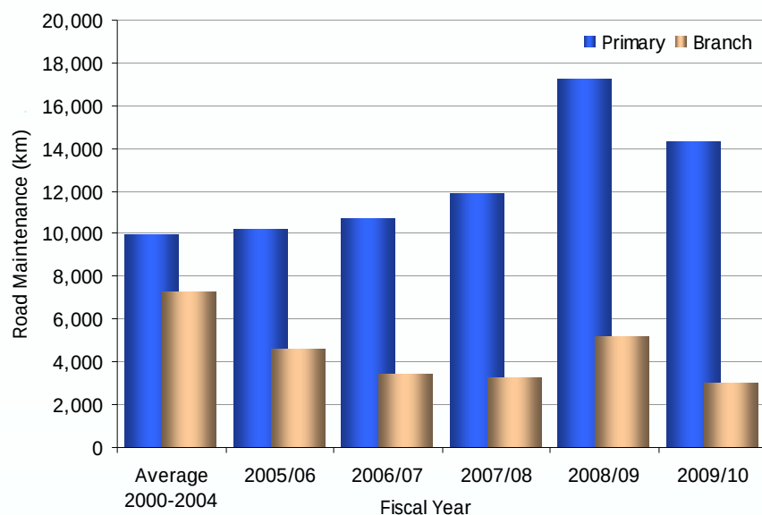
Figure 8b - Total Road Maintenance by Road Class by Year
