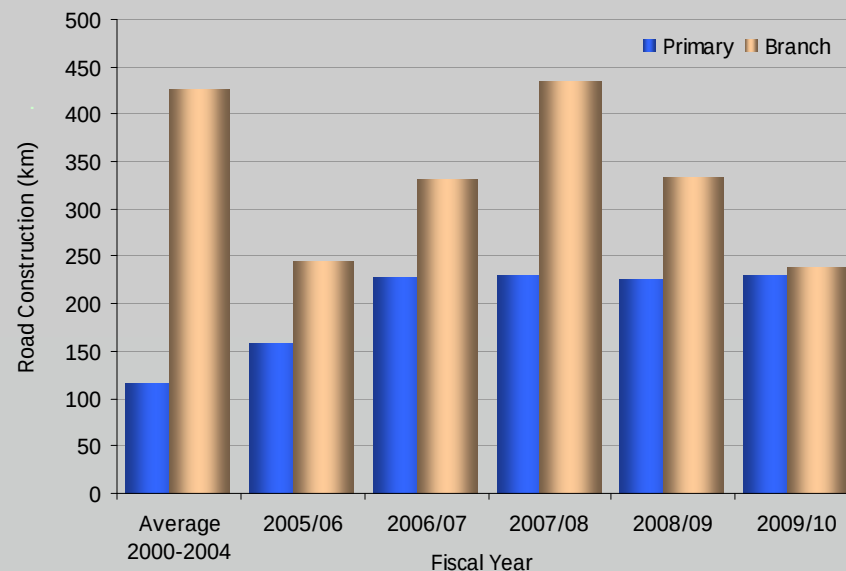
Figure 8a - Primary and Secondary Road Construction by Year
