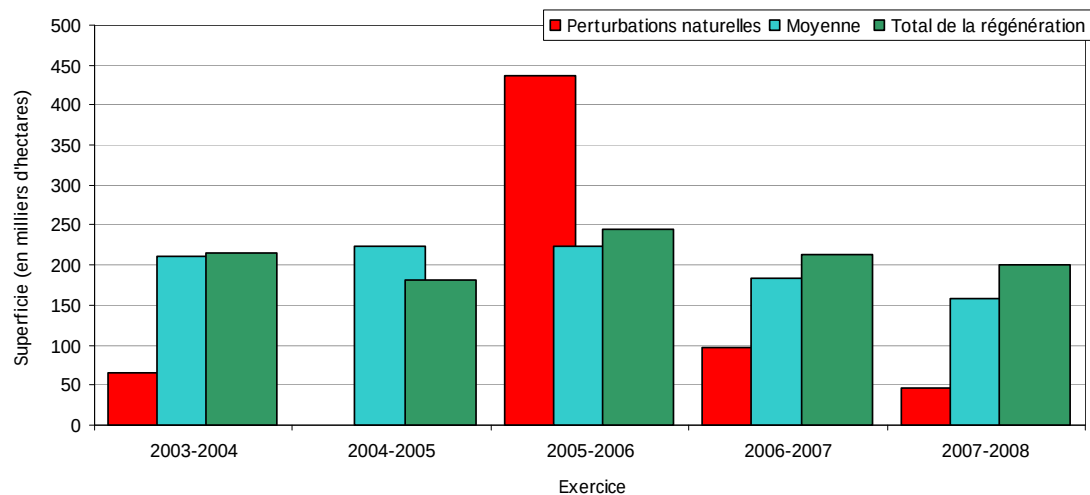
Figure 5a – Zone de perturbation naturelle (incendie et chablis), Perturbation naturelle
