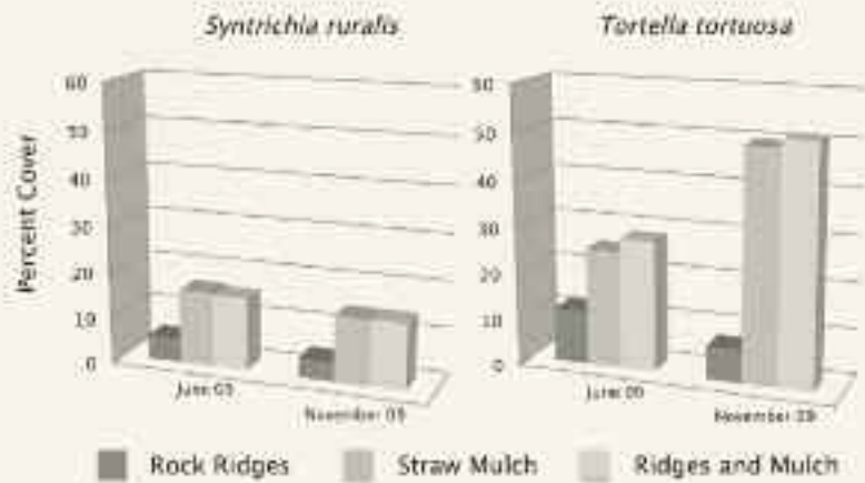
Figure 3: Effect of topography and mulch on moss establishment on a limestone quarry floor. The experiment was initiated in November 2008.
