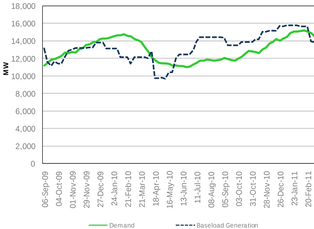
Figure 6.1 Minimum Demand and Baseload Generation
