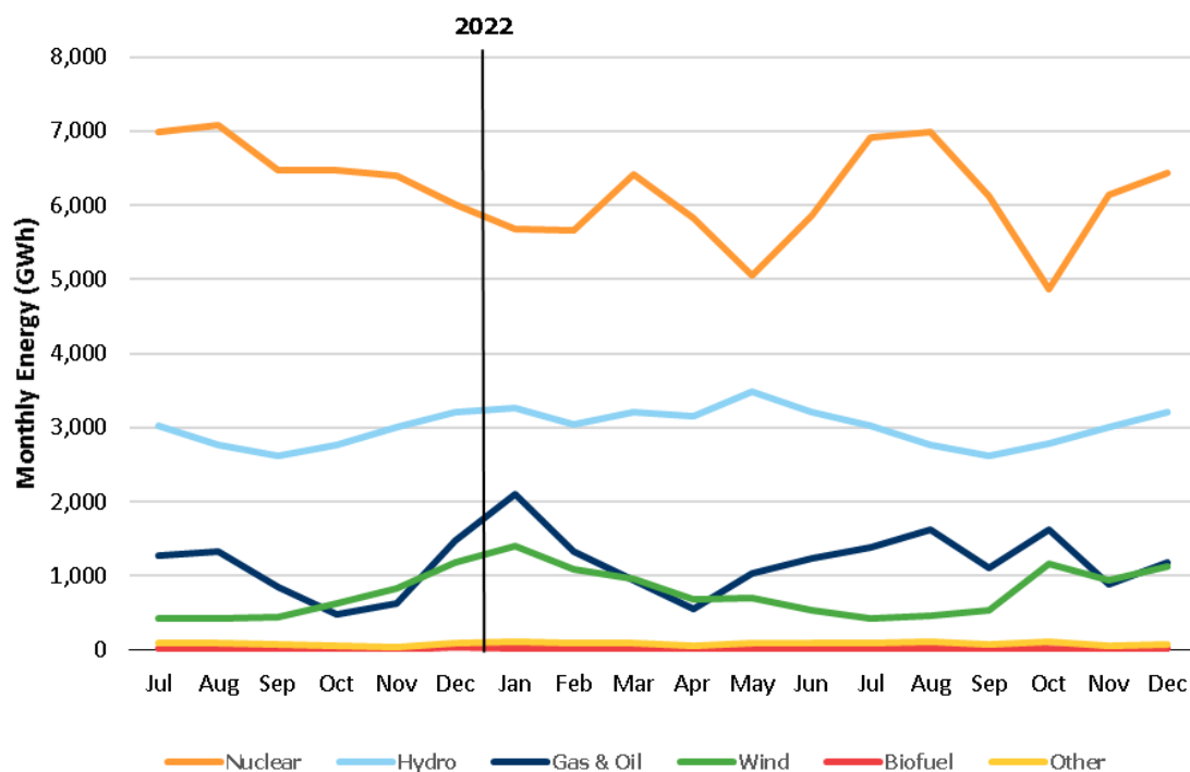
Figure 4-7 | Forecast Monthly Energy Production by Fuel Type
