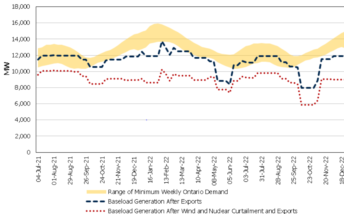
Figure 6-2 | Minimum Ontario Demand and Baseload Generation
