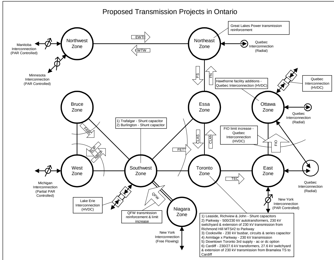
Figure 4.2 Potential New Transmission Facilities in Ontario
