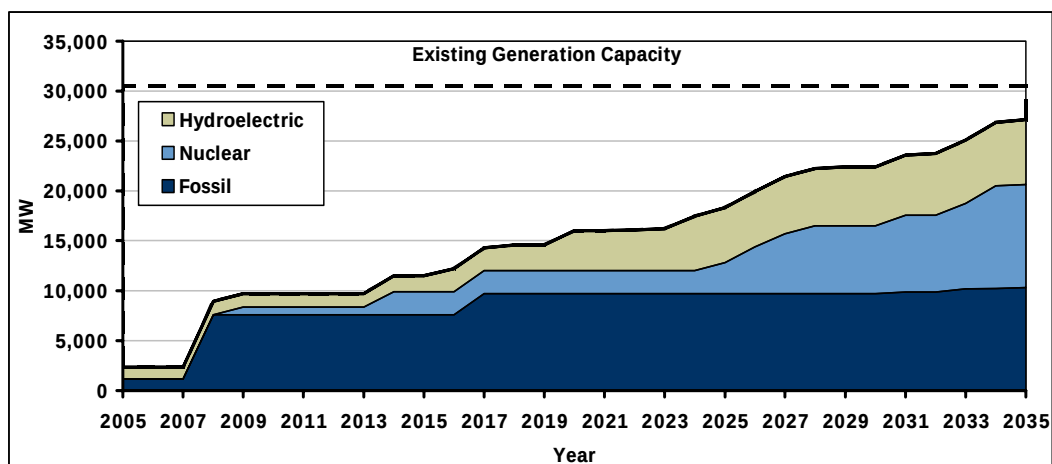
Figure 3.4 Capacity Exceeding Nominal Life, Retiring, Or In Need Of Major Refurbishment
