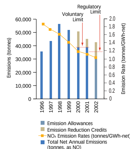
Figure 3 NO x Emissions and NO x Emission Rate for OPG Fossil Generation (1996-2002)
