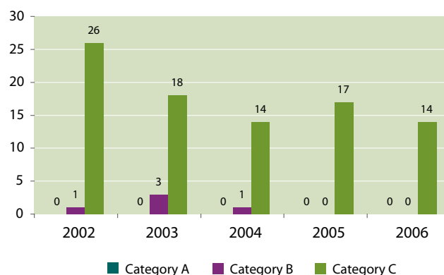
Figure 2: Spills Performance 2002 - 2006 1
