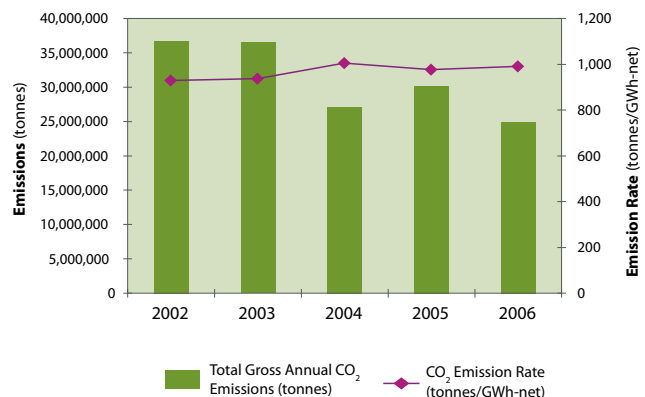
Figure 7: CO 2 Emissions and CO 2 Emission Rates for Fossil Generation 2002 - 2006
