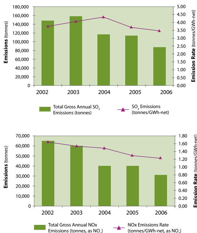
Figure 6: SO 2 and NO x Emissions and Emission Rates for OPG Fossil Generation (2002 – 2006).
