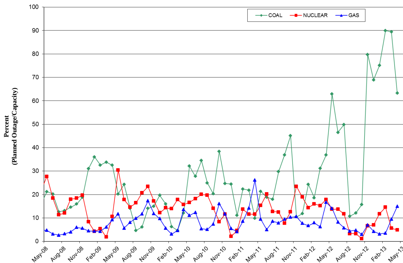
Figure 1-23: Planned Outages Relative to Capacity by Fuel Type May 2008 – April 2013 (% of capacity)
