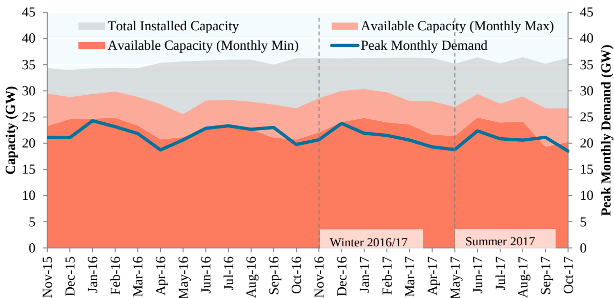
Figure A-22: Unavailable Generation Relative to Installed Capacity November 2015 – October 2017 (GW)
