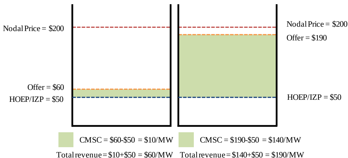
Figure 2-2: Demonstration of Nodal Price Chasing ($/MW)
