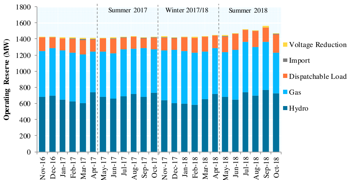
Figure A-22: Average Hourly OR Scheduled by Resource Type
