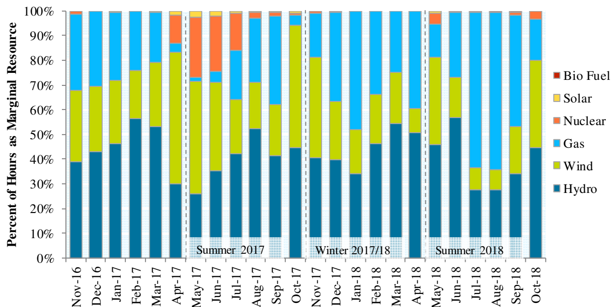
Figure A-7: Share of Resource Type Setting the Real-Time MCP
