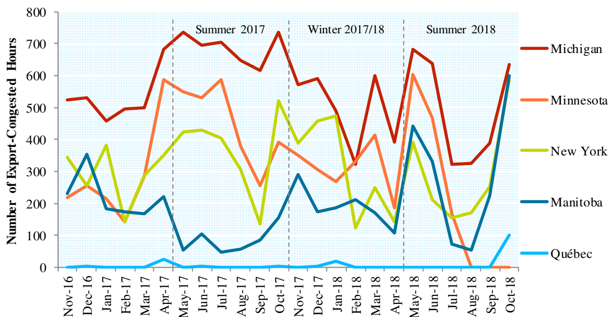
Figure A-16: Export Congestion by Intertie
