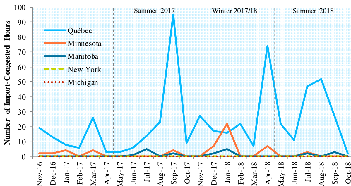
Figure A-15: Import Congestion by Intertie
