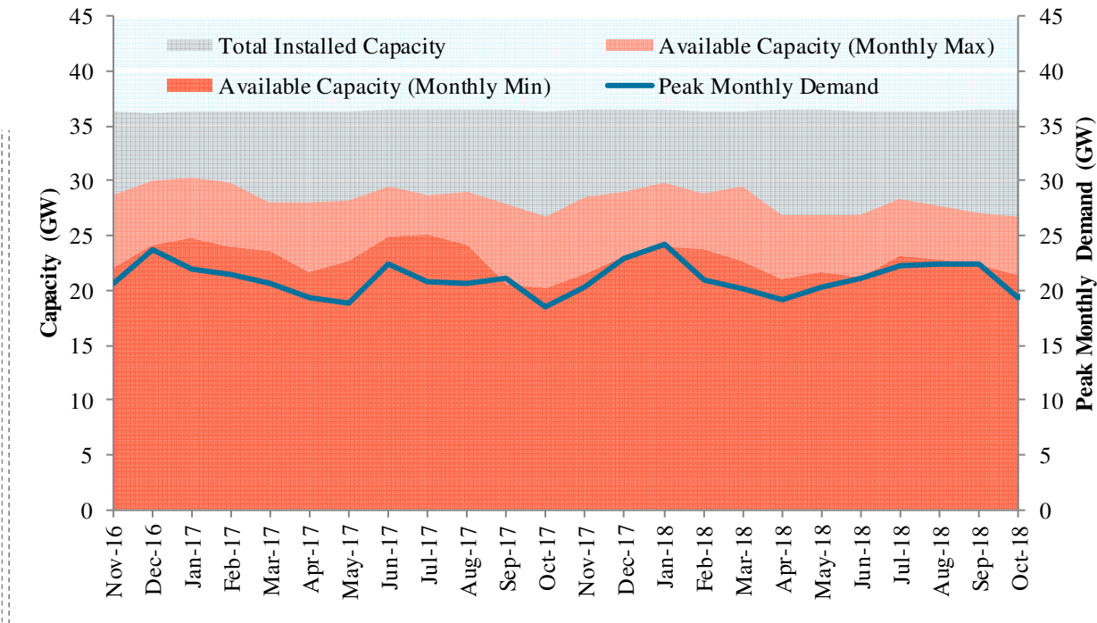
Figure A-23: Unavailable Generation Relative to Installed Capacity
