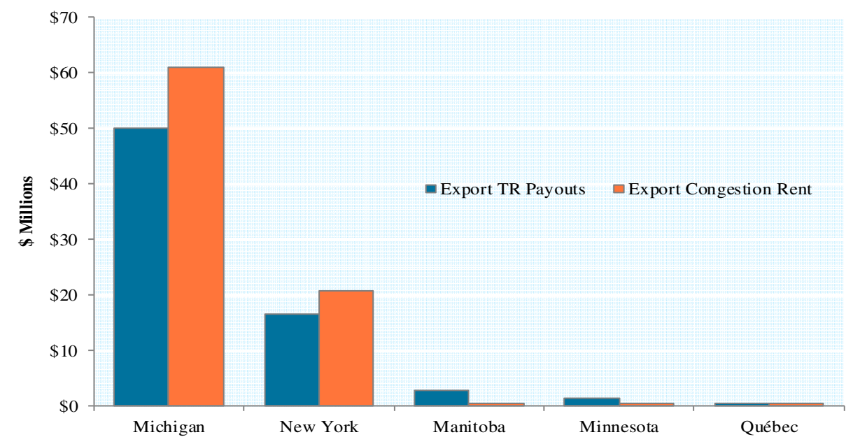
Figure A-18: Export Congestion Rent & TR Payouts by Intertie
