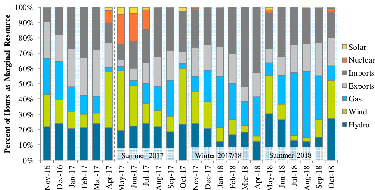
Figure A-8: Share of Resource Type Setting the One-Hour Ahead Pre-Dispatch MCP
