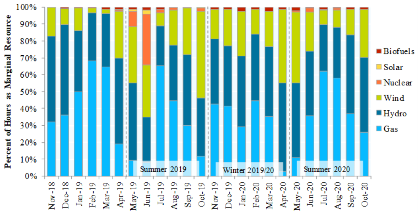
Figure A-7: Share of Resource Type Setting the Real-Time MCP, 2 Years
