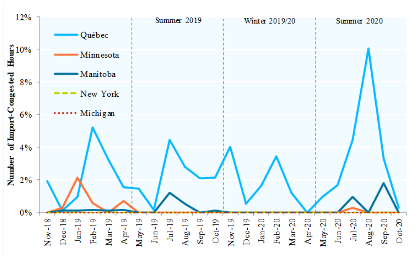
Figure A-15: Import Congestion by Intertie, 2 Years
