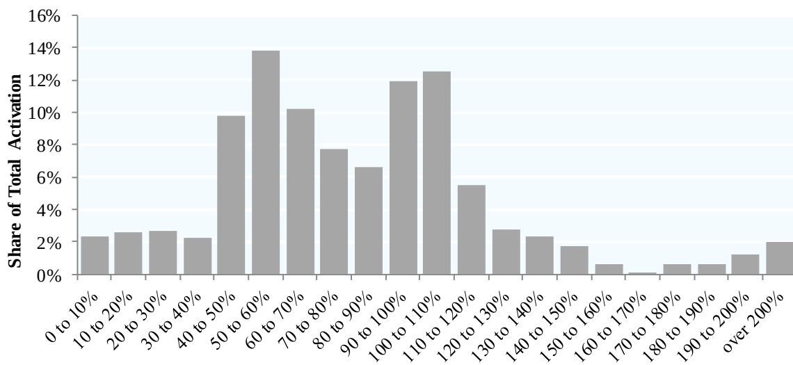
Figure 3-1: Distribution of HDR Performance (Energy Delivered/Activated) for July 9 and 10, 2020
