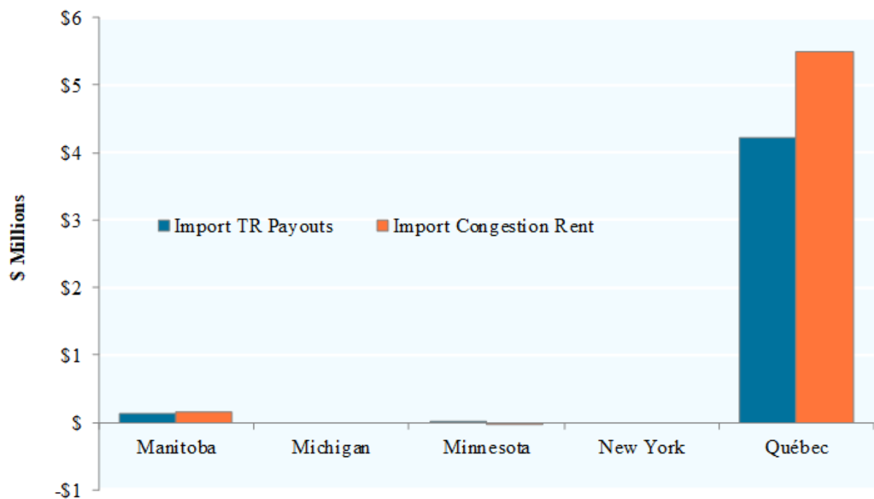
Figure A-17: Import Congestion Rent & Transmission Rights (TR) Payouts by Intertie, 1 Period
