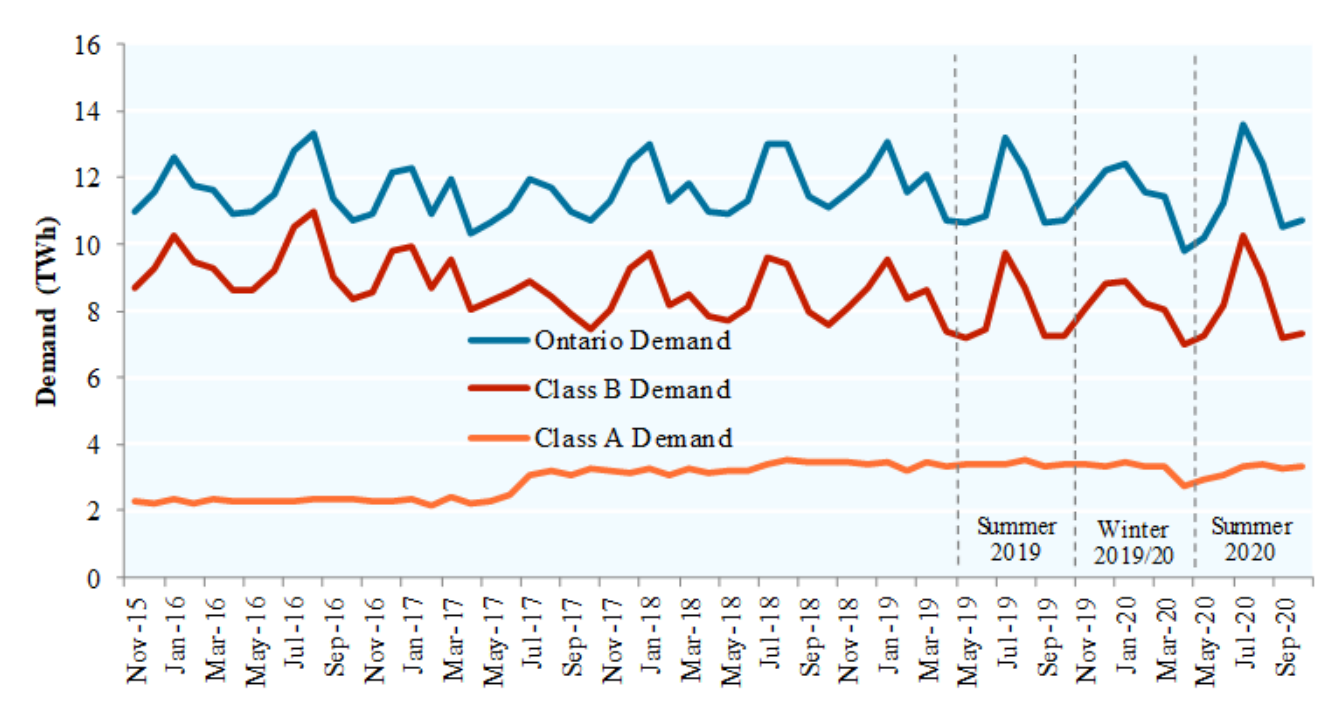
Figure A-20: Monthly Ontario Energy Demand by Class A &amp; Class B Consumers, 5 Year
