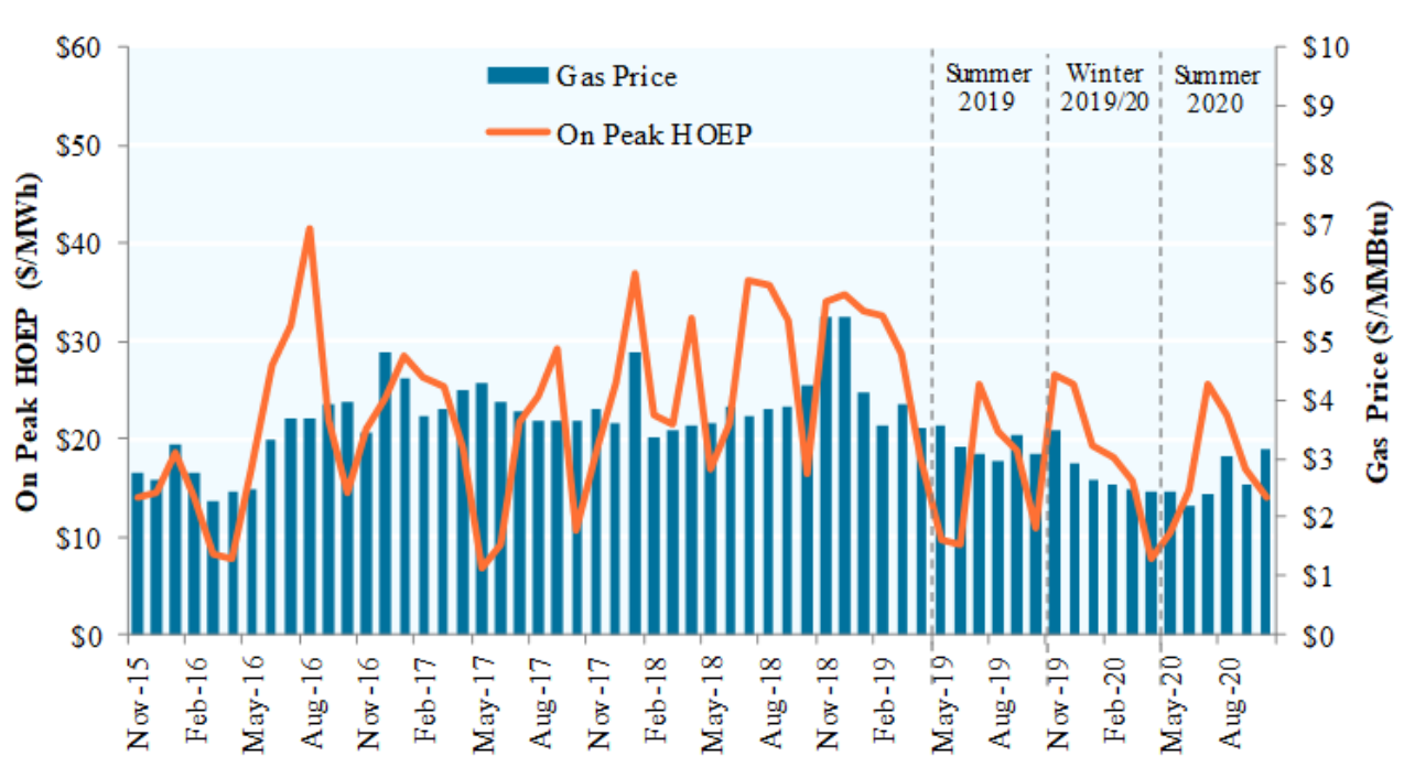
Figure A-5: Natural Gas Price &amp; HOEP during Peak Hours, 5 Years
