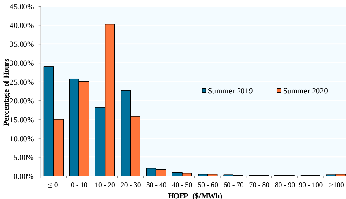
Figure A-6: Frequency Distribution of HOEP, 2 Periods
