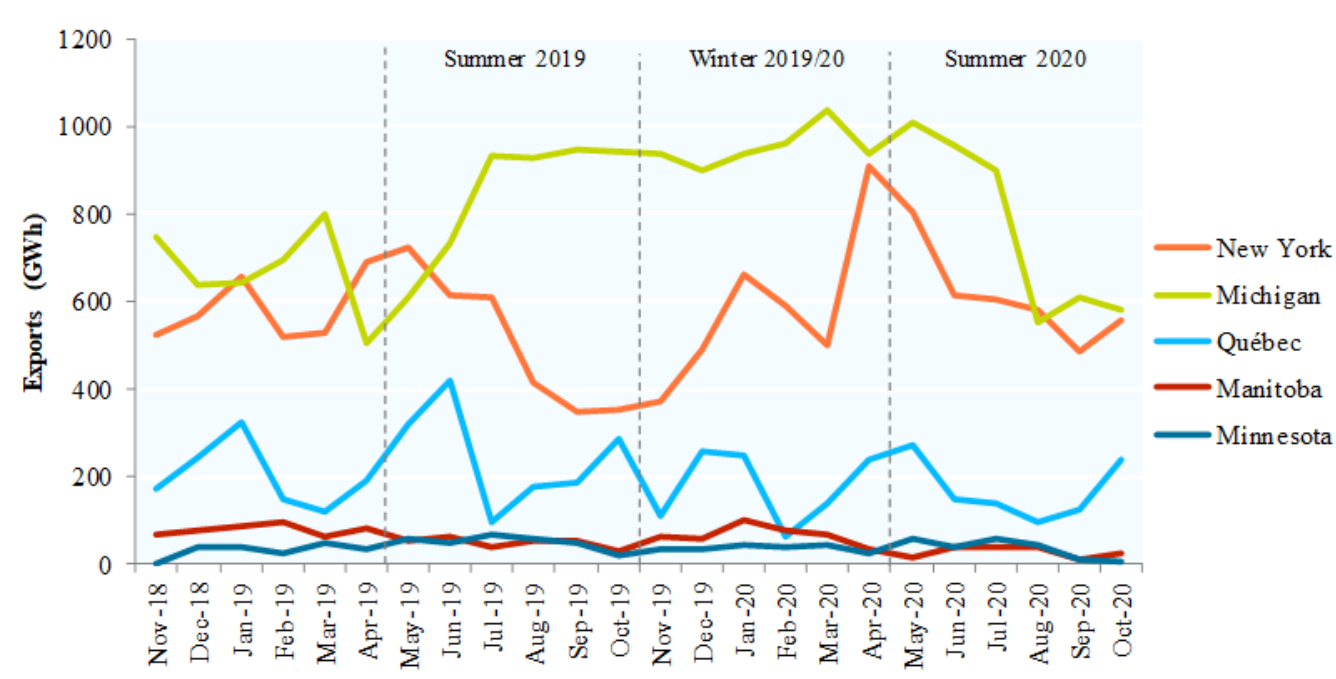
Figure A-25: Exports by Intertie, 2 Years
