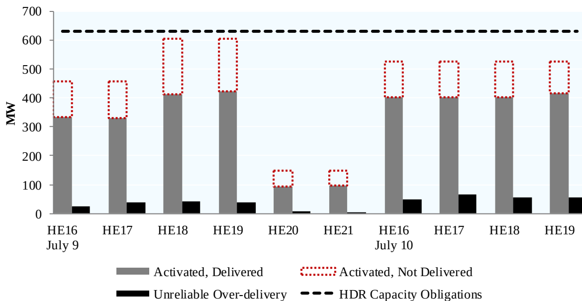
Figure 3-2: HDR Performance for July 9 and 10, 2020
