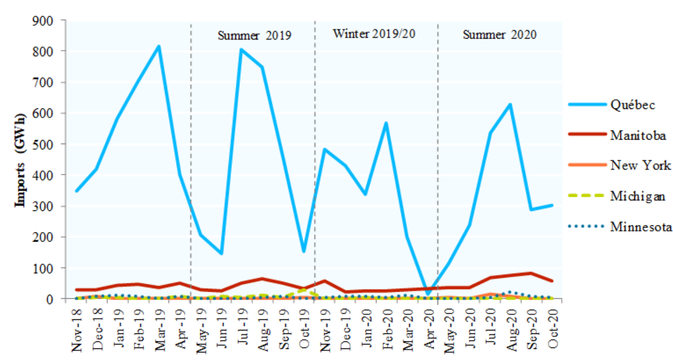
Figure A-26: Imports by Intertie, 2 Years
