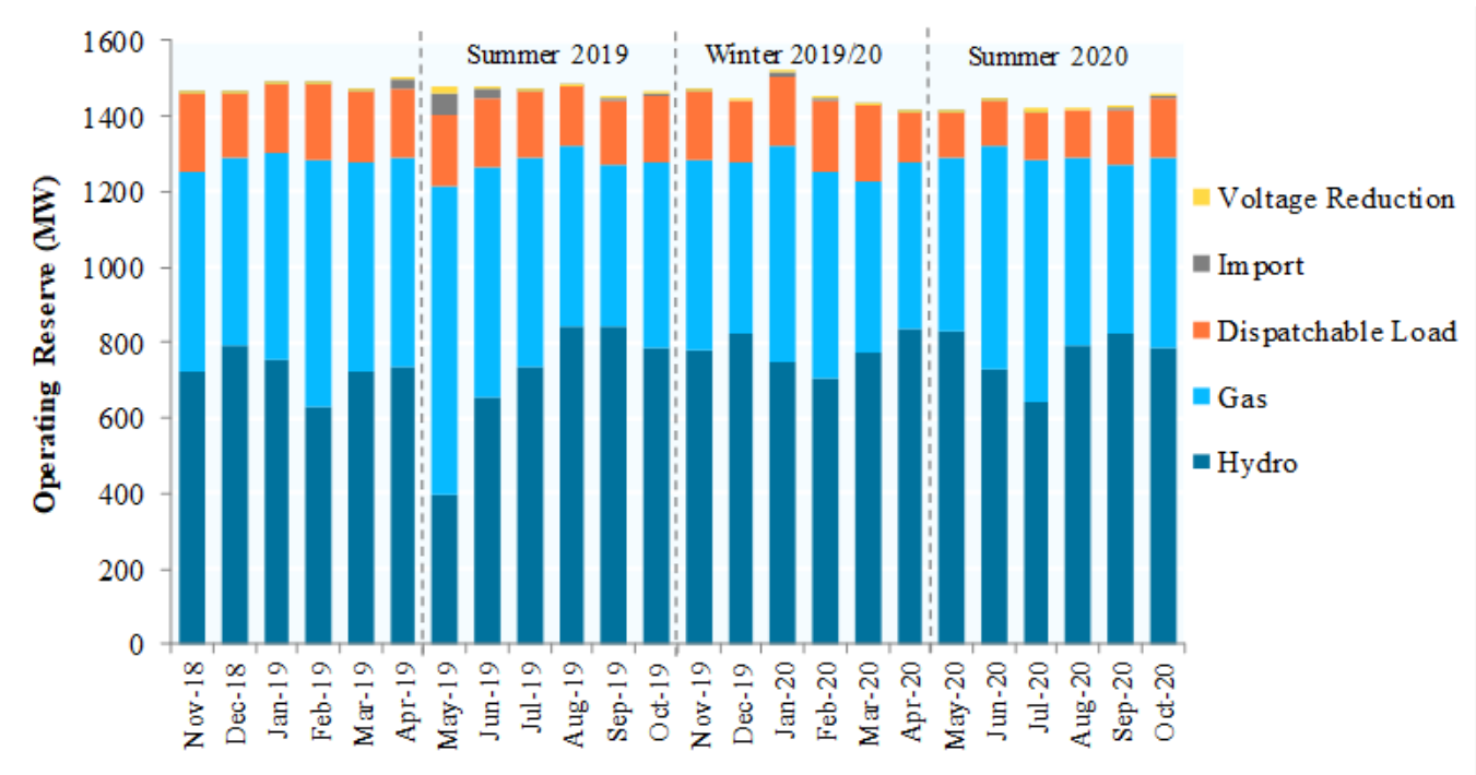
Figure A-22: Average Hourly OR Scheduled by Month and Resource Type, 2 Years
