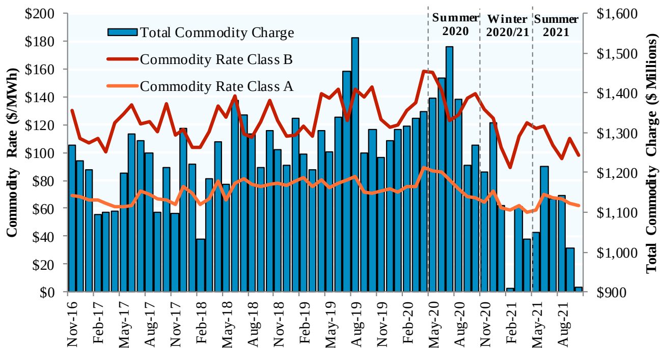
Figure A-26: Monthly Average Commodity Rate &amp; Commodity Charges, 5 Years
