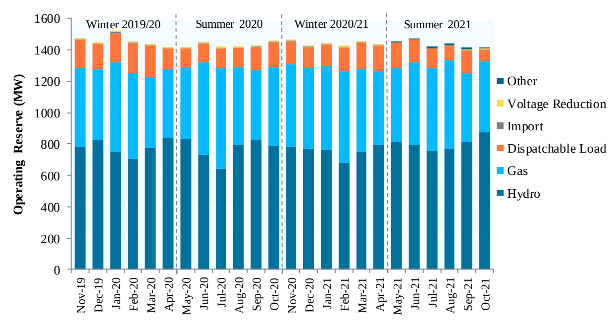
Figure A-17: Average Hourly OR Scheduled by Resource Type, 2 Years
