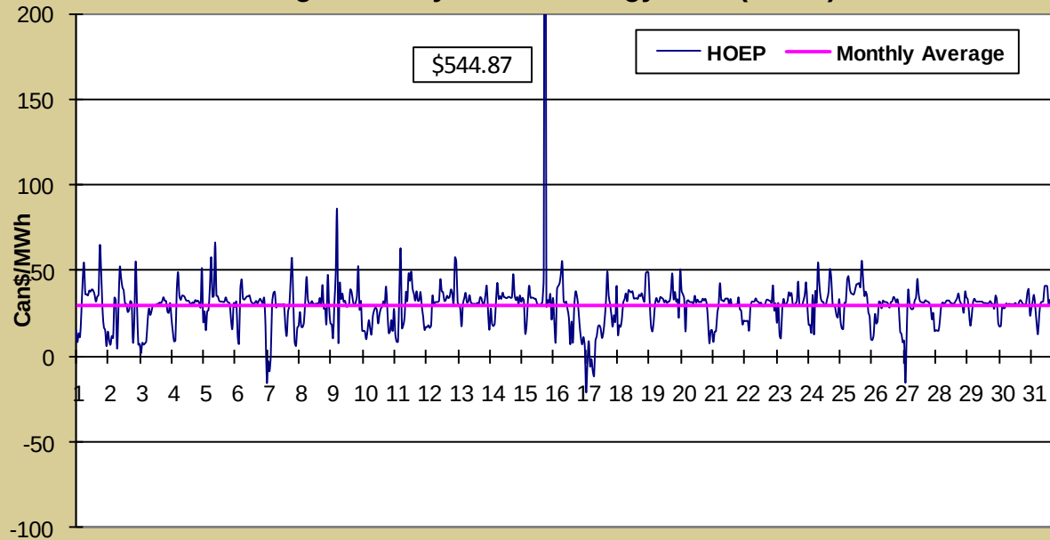
Fig 1 - Hourly Ontario Energy Price (HOEP)
