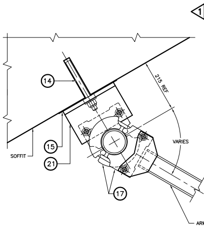
HINGE CONNECTION AT SOFFIT
