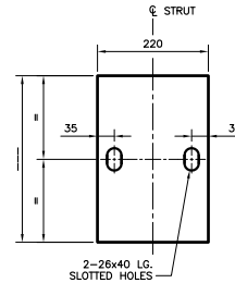
13 CONNECTING PLATE DETAIL
