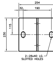
21 CONNECTING TEE DETAIL
