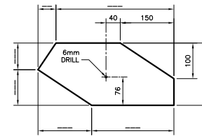
6 GUSSET DETAIL
