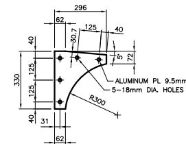
DAMPER GUSSET
