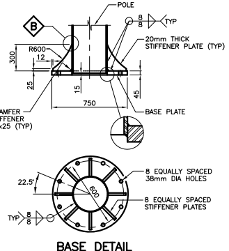
BASE DETAIL
