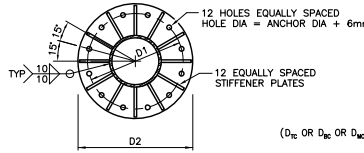
BASE DETAIL NOTE: FOR ANCHOR DIMENSIONS D1 AND D2, SEE FOOTING DRAWING FOR DETAILS.
