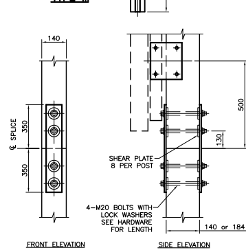
POST SPLICE DETAIL - TYPE "A"
