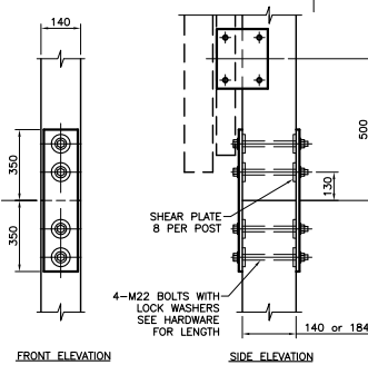
POST SPLICE DETAIL - TYPE "B"
