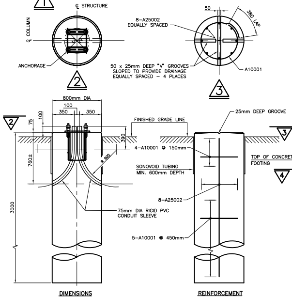
FOOTING DETAILS
