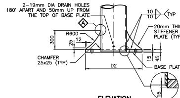
ELEVATION LEG DETAIL
