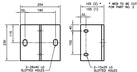
1 2 CONNECTING TEE DETAIL
