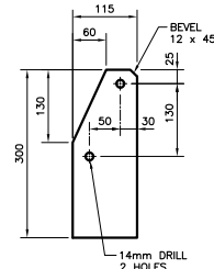
5 POST CARRIER DETAIL
