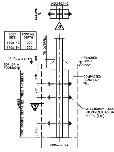
FOOTING DETAILS
