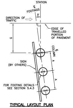
TYPICAL LAYOUT PLAN
