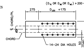
TYPICAL CHORD CONNECTION PLATE
