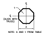
ALTERNATIVE LEG SECTION
