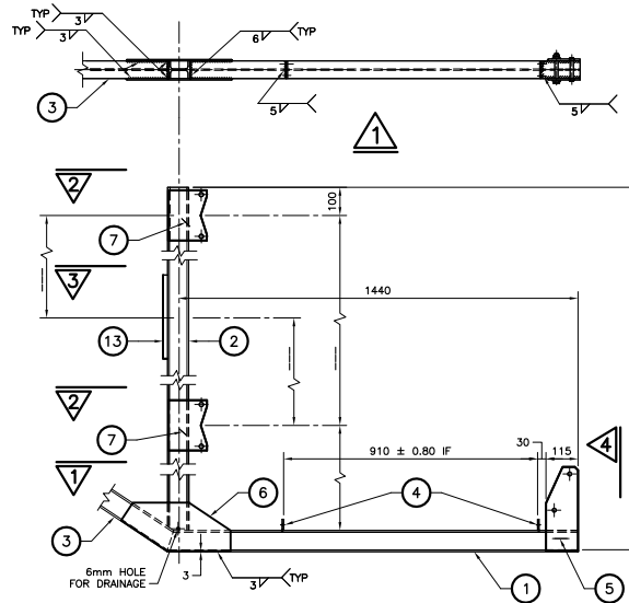
ARM DETAIL
