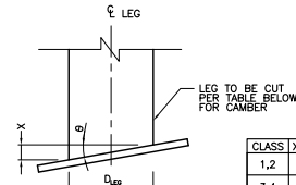
DETAIL FOR CAMBER
