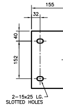
21 CONNECTING TEE DETAIL
