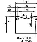
7 GUSSET DETAIL
