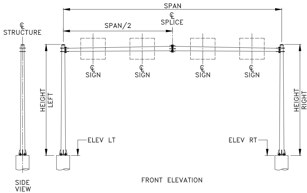
FIGURE 7.1.2(a) TYPE I – FRONT MOUNTED
