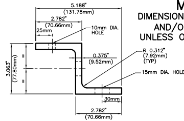
ALUMINUM Z-BRACKET
