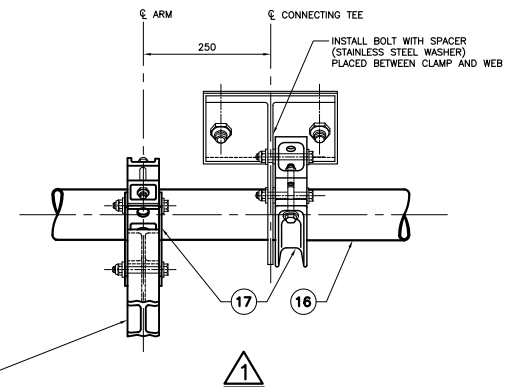
HINGE CONNECTION AT SOFFIT
