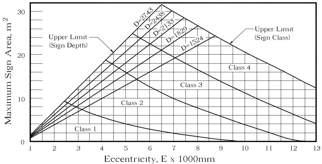
FIGURE 3.2.2(b) CLASS RANGES FOR 325 \text{ Pa} < q \leq 425 \text{ Pa} (Single Cantilever Sign Support)
