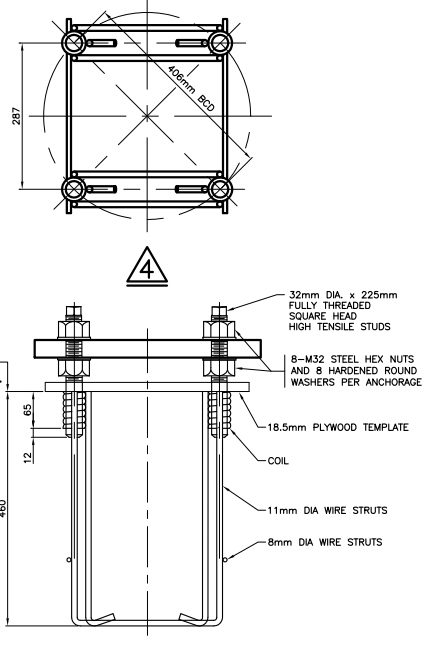
ANCHORAGE DETAILS
