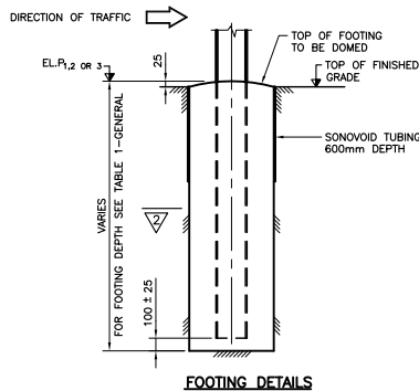
FOOTING DETAILS
