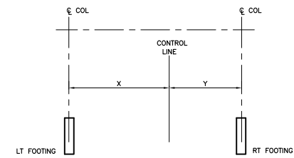
FRONT ELEVATION FOOTING LAYOUT DETAILS
