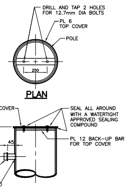
TOP PLATE DETAIL SIDE ELEVATION
