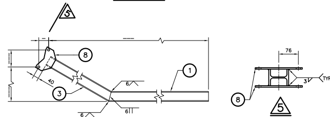
ARM DETAIL
