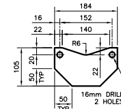
8 GUSSET DETAIL
