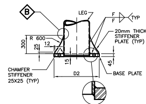
BASE DETAIL
