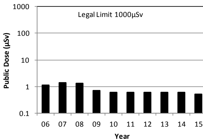
Figure 4-2: Darlington Nuclear Annual Public Dose Trend
