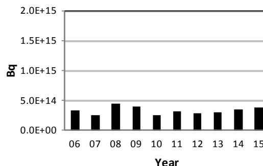
Figure 2-7: Pickering Nuclear Tritium Oxide Water Emissions
