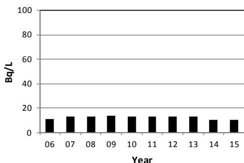
Figure 3-25: DN Annual Average HTO in Well Water
