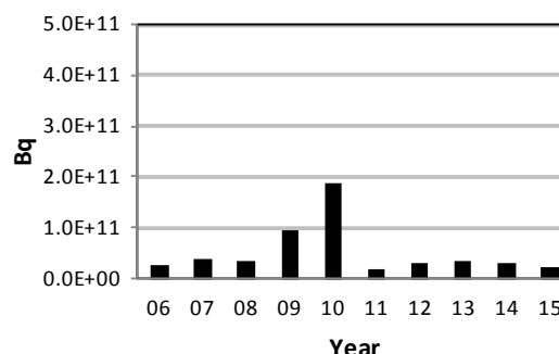
Figure 2-9: Pickering Nuclear Gross Beta-Gamma Water Emissions
