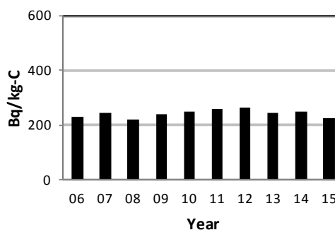
Figure 3-32: PN Annual Average C-14 in Fish
