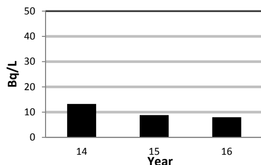
Figure 3-16: DN Annual Average HTO in Poultry
