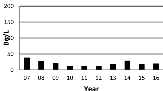
Figure 3-6: DN Annual Average HTO in Vegetation
