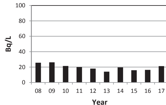
Figure 3-28: PN Annual Average HTO in Lake Water
