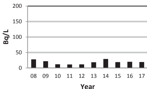
Figure 3-6: DN Annual Average HTO in Vegetation
