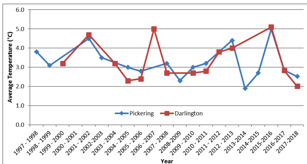
Figure 3-36: Long term trends in Lake Ontario winter temperatures (Dec 15th to January 15th)
