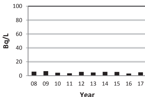
Figure 3-29: DN Annual Average HTO in Fish
