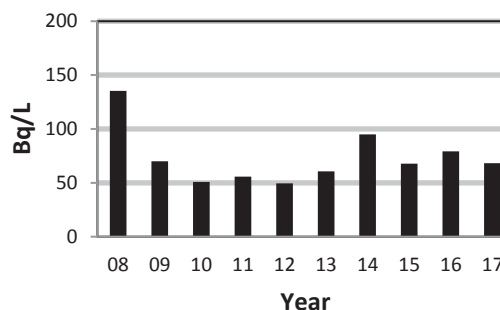
Figure 3-7: PN Annual Average HTO in Vegetation
