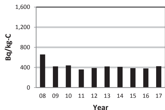
Figure 3-4: PN Annual Average C-14 in Air
