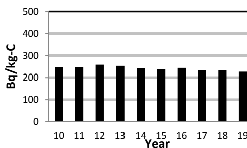
Figure 3-13: PN Annual Average C-14 in Milk
