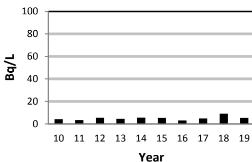
Figure 3-29: DN Annual Average HTO in Fish
