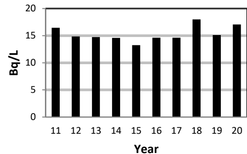
Figure 3-11: PN Annual Average HTO in Milk
