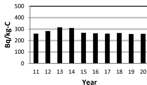
Figure 3-9: PN Annual Average C-14 in Vegetation
