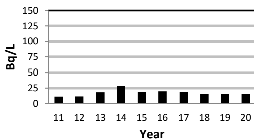
Figure 3-6: DN Annual Average HTO in Vegetation
