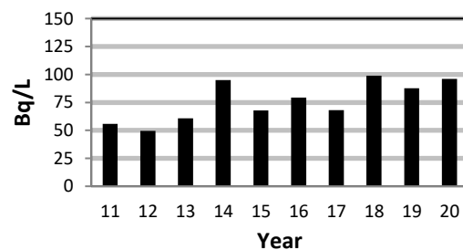
Figure 3-7: PN Annual Average HTO in Vegetation
