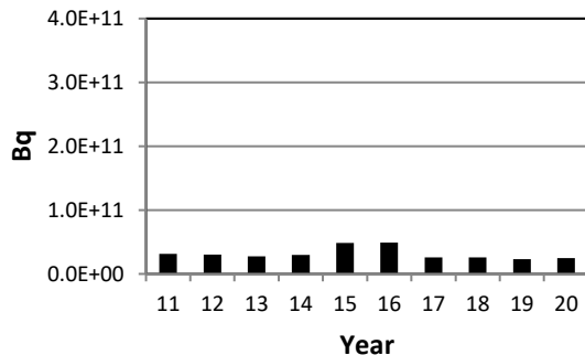
Figure 2-8: Darlington Nuclear Gross Beta-Gamma Water Emissions
