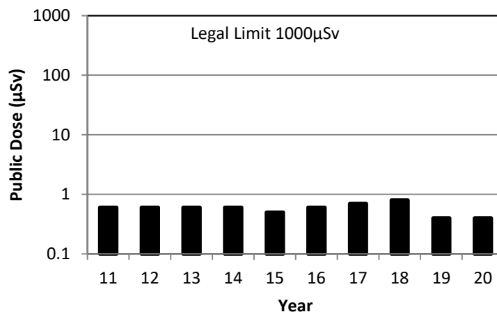
Figure 4-2: Darlington Nuclear Annual Public Dose Trend
