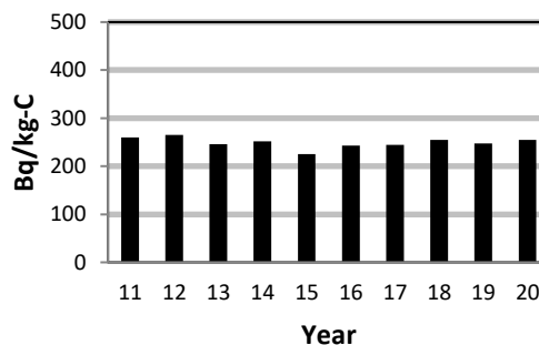
Figure 3-32: PN Annual Average C-14 in Fish
