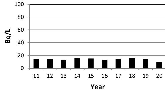
Figure 3-26: PN Annual Average HTO in Well Water
