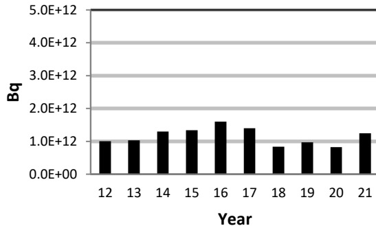
Figure 2-4: Darlington Nuclear C-14 Air Emissions
