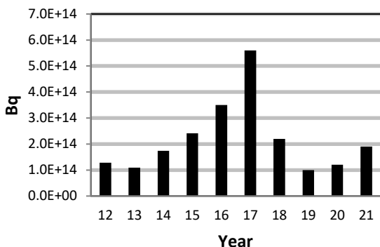
Figure 2-6: Darlington Nuclear Tritium Oxide Water Emissions
