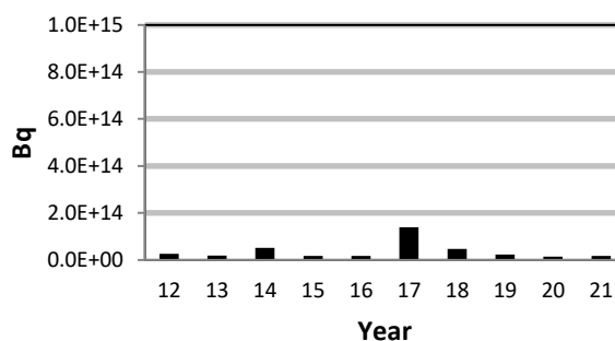
Figure 2-1: Darlington Nuclear Airborne Elemental Tritium Emissions
