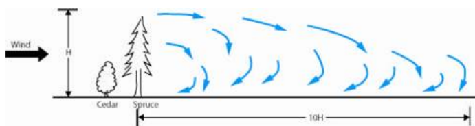
Figure 1. Porous windbreaks, such as this tree shelterbelt give good protection for a horizontal distance of about 10X their height.
