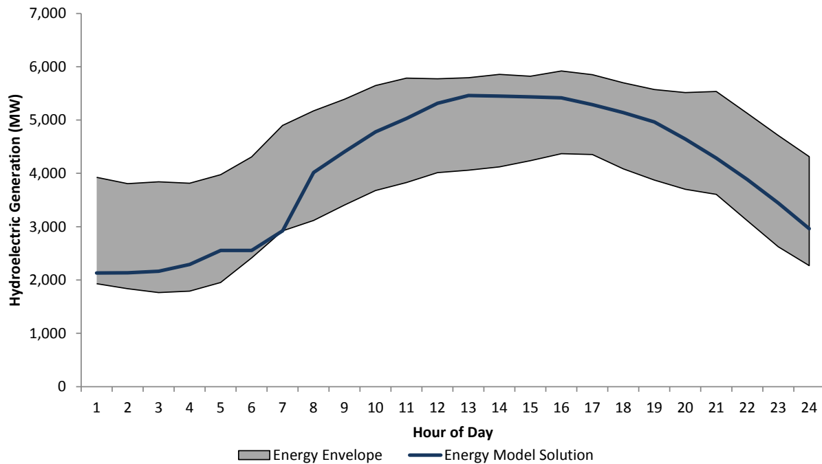
Figure 3.6 Hydroelectric Solution for a Particular Weekday vs. Hourly and Daily Energy Constraints
