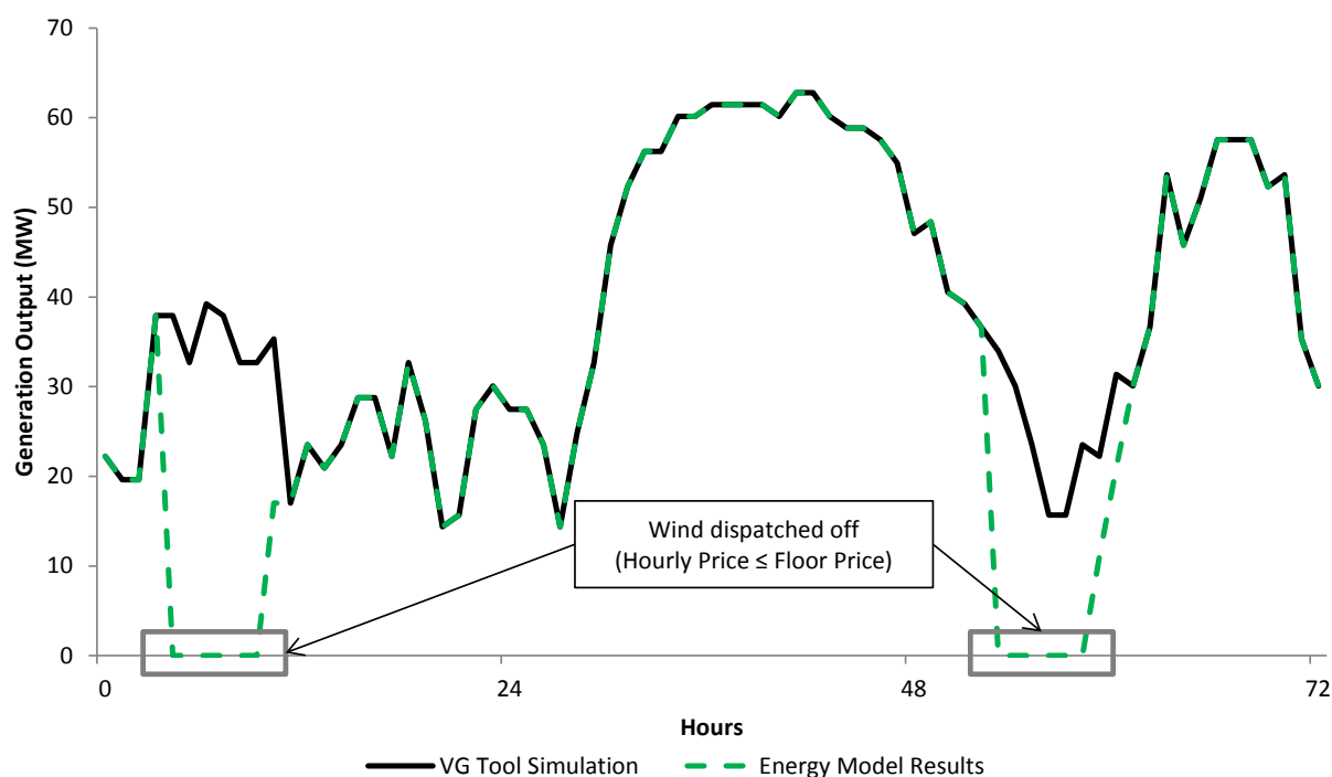
Figure 3.7 Wind Simulation versus Energy Model Dispatch for a Particular Unit
