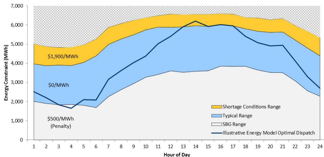
Figure 3.6 Hydroelectric Solution for a Particular Weekday vs. Hourly and Daily Energy Constraints
