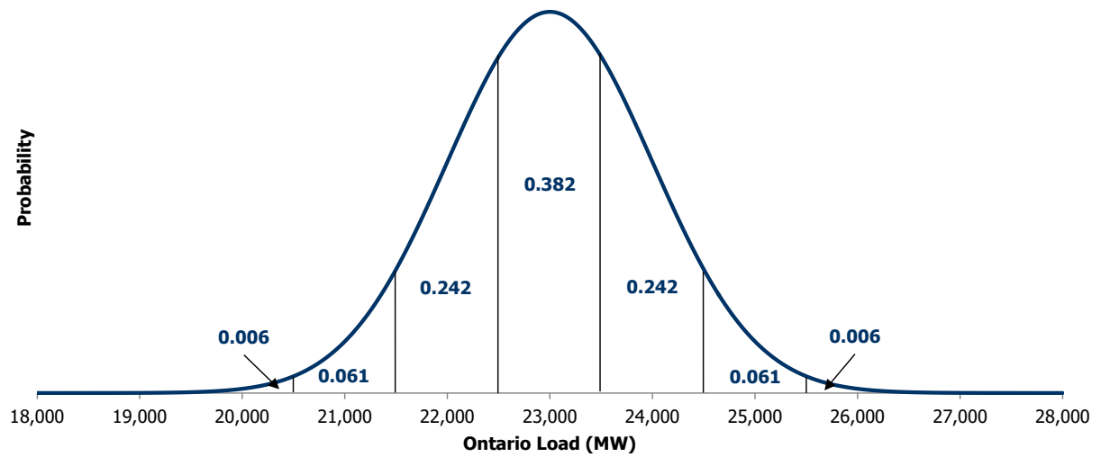
Figure 4-3 | Seven-Step Approximation of Normal Distribution - Example
