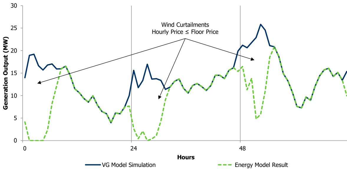
Figure 6-4 | Wind Simulation versus Energy Model Dispatch for a Particular Unit
