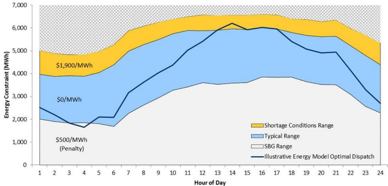
Figure 5-3 | Hydroelectric Solution for a Particular Weekday vs. Hourly and Daily Energy Constraints
