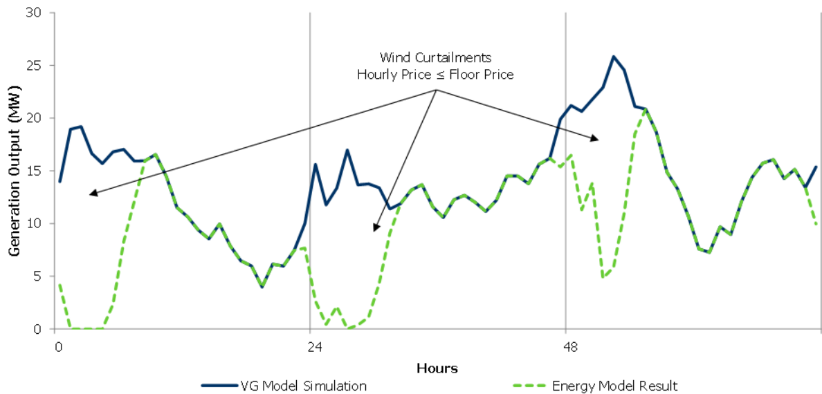
Figure 5-4 | Wind Simulation versus Energy Model Dispatch for a Particular Unit
