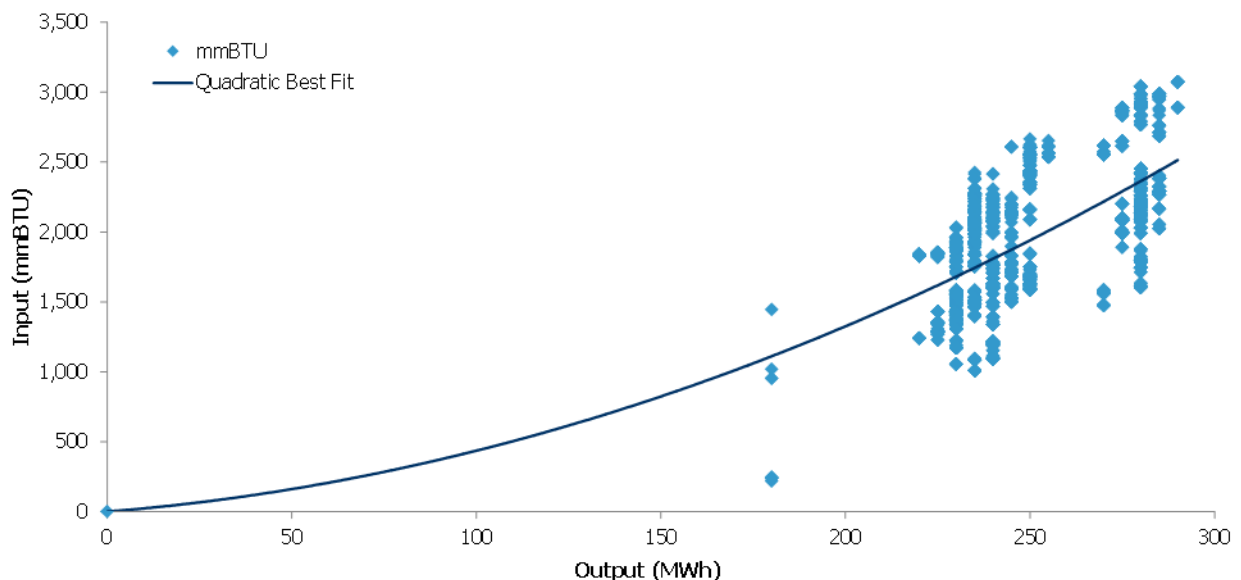
Figure 5-1 | Quadratic Best Fit I-O Equation for a Particular Combustion Generator
