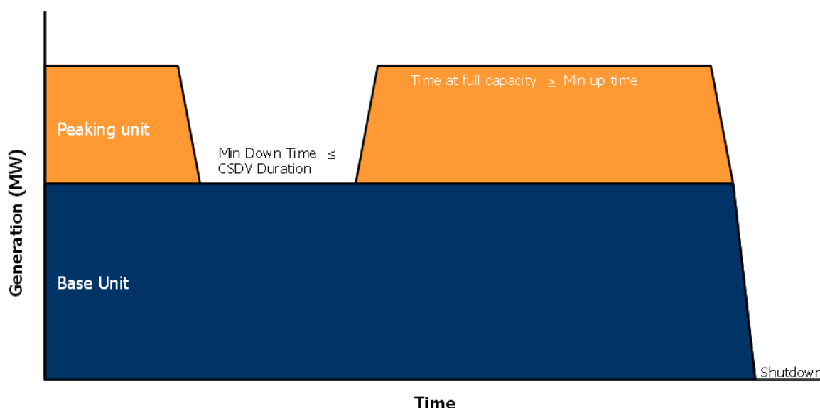
Figure 5-2 | Nuclear Manoeuvring Unit Dispatch Illustration
