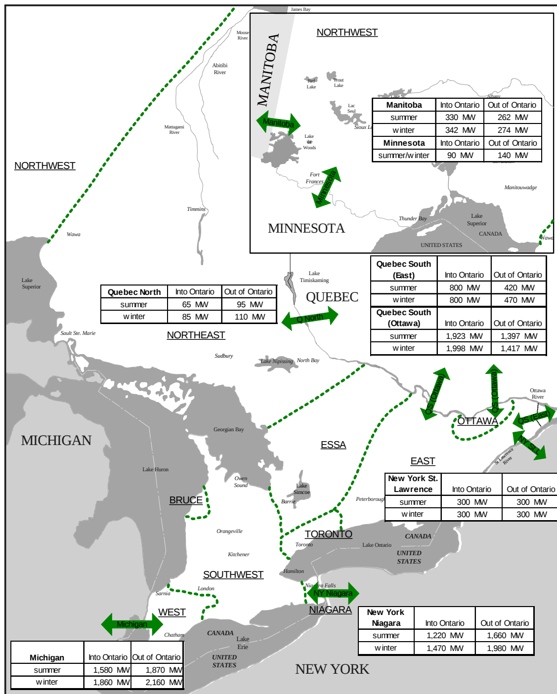
Figure 2.1.2 Ontario's Points of Interconnection with Neighbouring Areas
