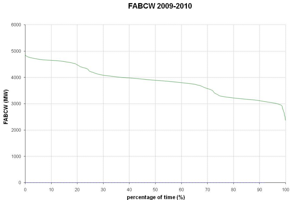
Figure 3.3.1 One Year Rolling Historical Flow Distribution – Interfaces
