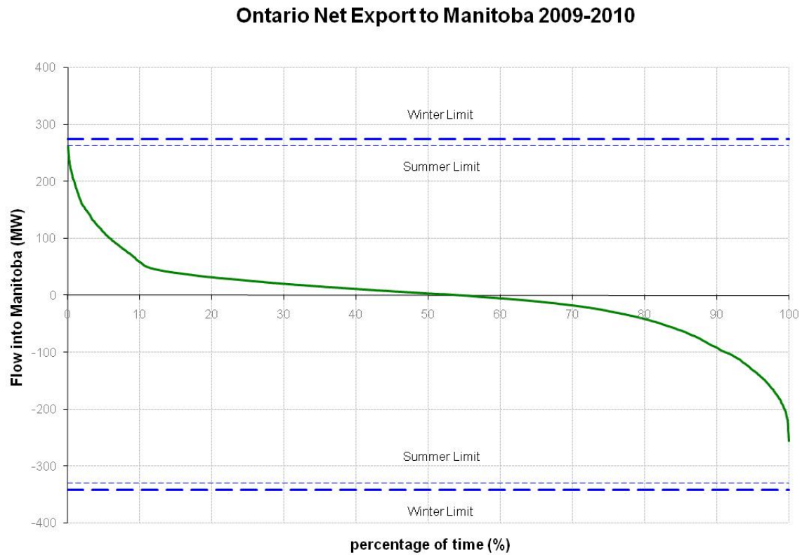
Figure 5.3.1 One Year Rolling Historical Flow Distribution – Interconnections
