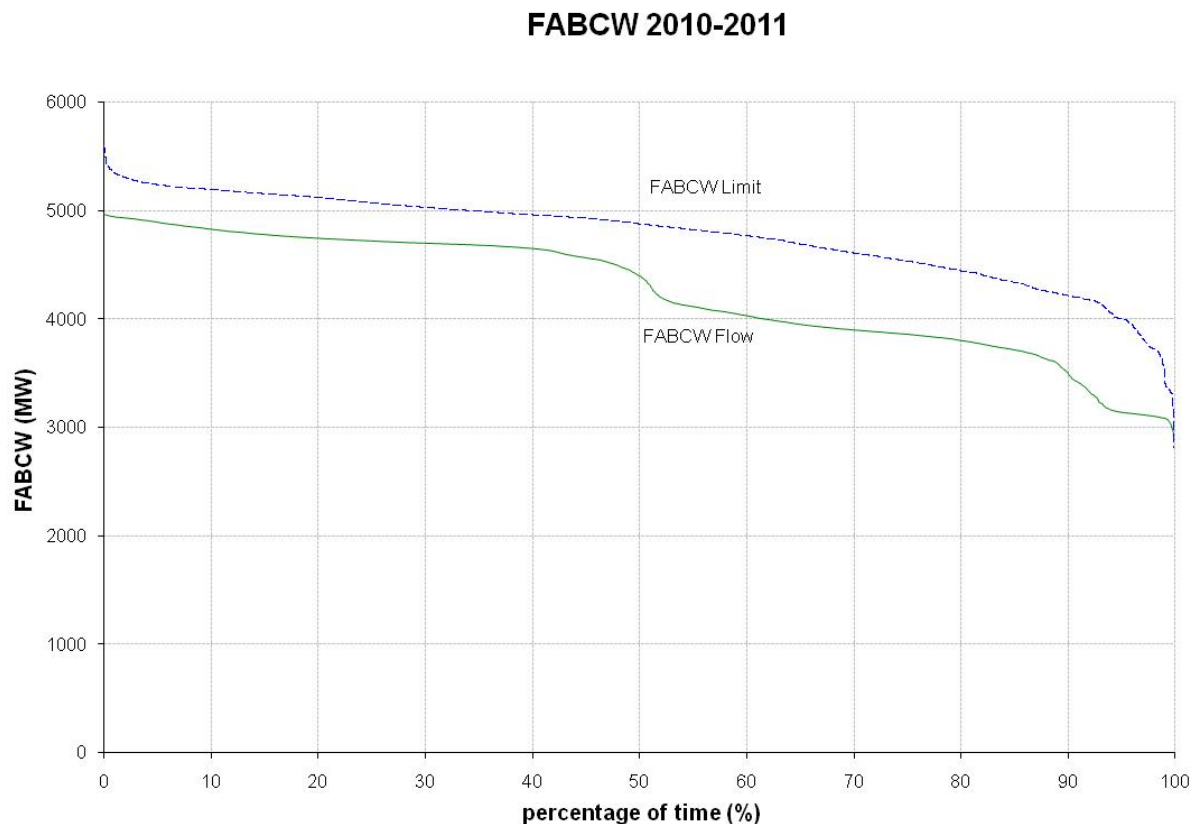
Figure 3.3.1 One Year Rolling (May 2010 – May 2011) Historical Flow Distribution - Interfaces
