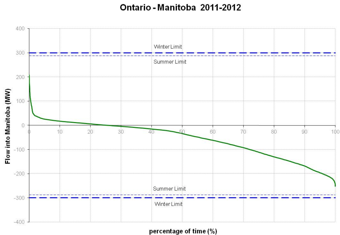
Figure 4.3.3 One Year Rolling (April 2011 – April 2012) Historical Flow Distribution - Interconnections
