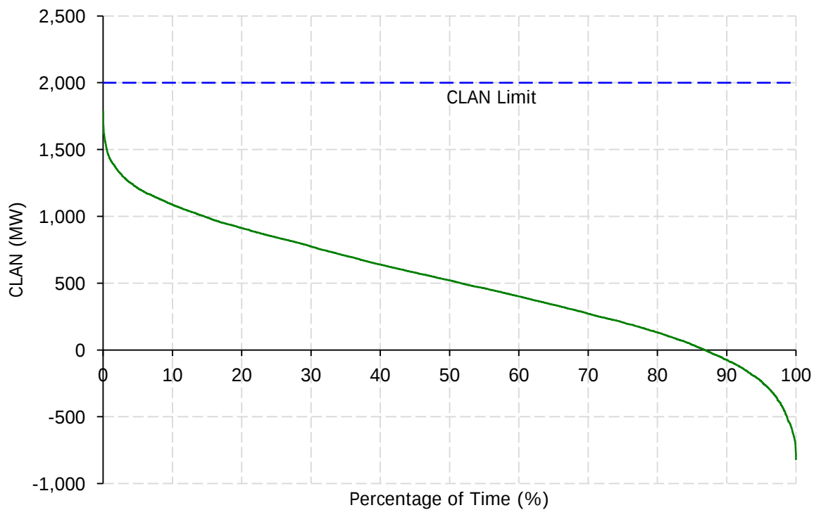
CLAN and CLAS Apr. 1, 2016 to Apr. 1, 2017
