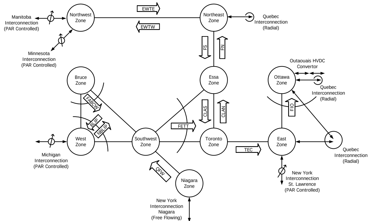
Figure 4.3.2 Ontario's Zones, Interfaces and Interconnections
