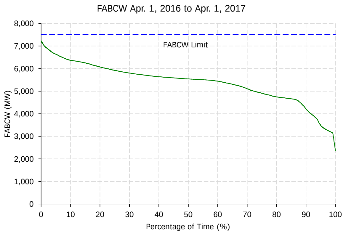
Figure 3.3.2 One Year Rolling (Apr. 2016 – Apr. 2017) Historical Flow Distribution - Interfaces
