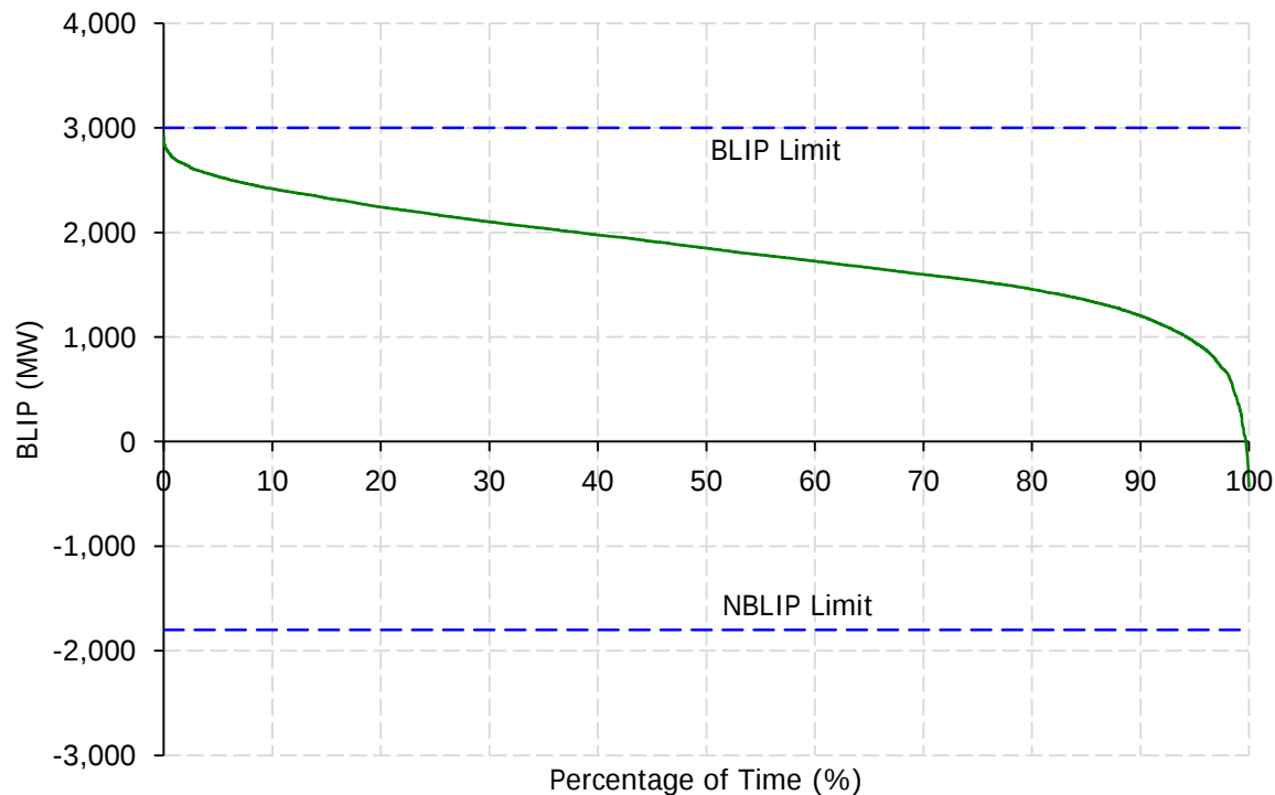
BLIP and NBLIP Apr. 1, 2016 to Apr. 1, 2017
