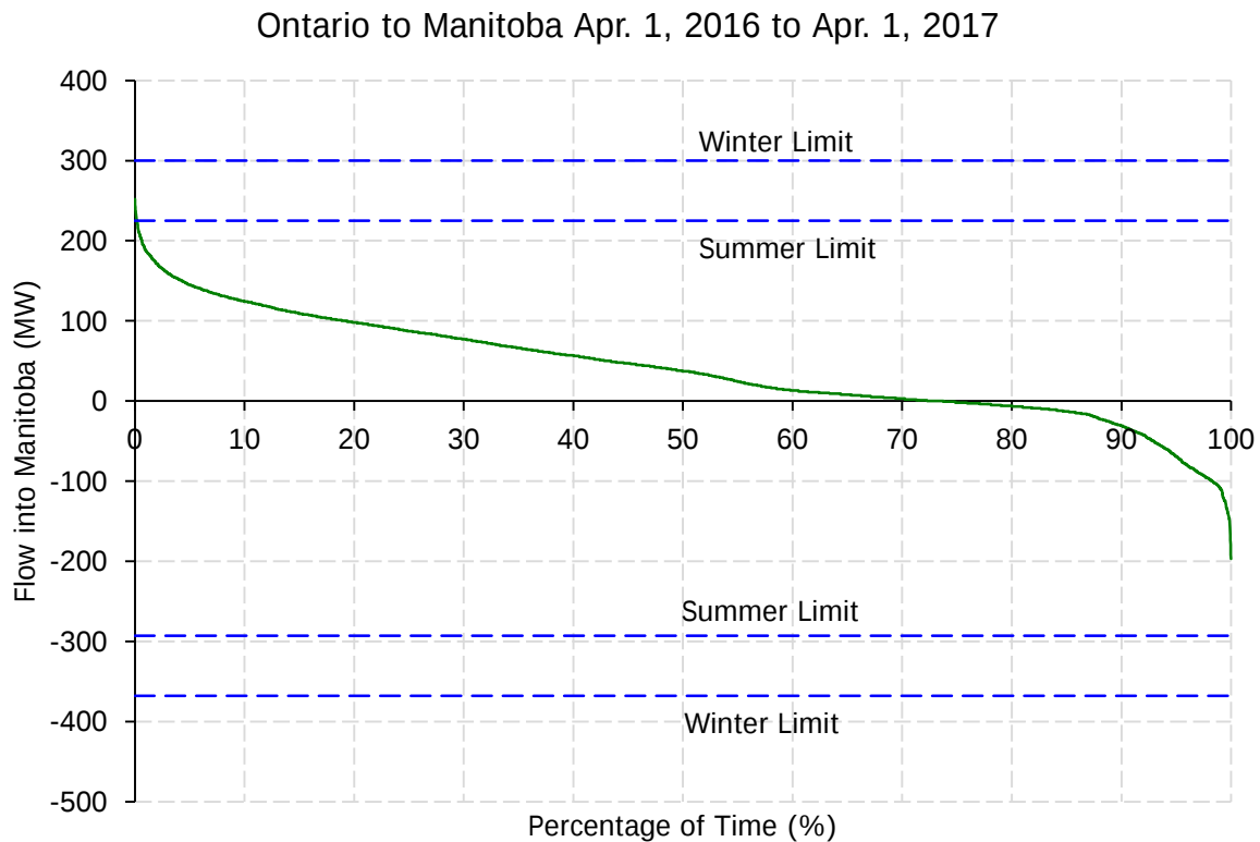
Figure 4.3.3 One Year Rolling (Apr. 2016 – Apr. 2017) Historical Flow Distribution - Interconnections
