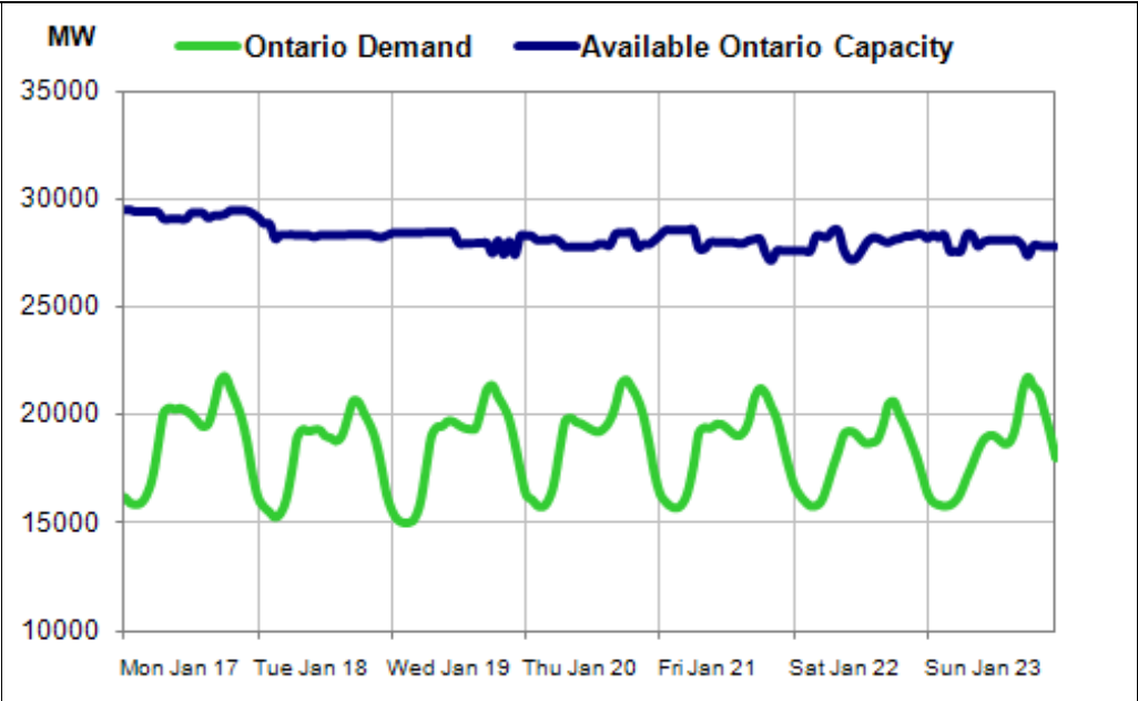
Hourly Ontario demand vs. available generation capacity within the province. Internal supply is supplemented by import capacity of up to 4,000 MW.
