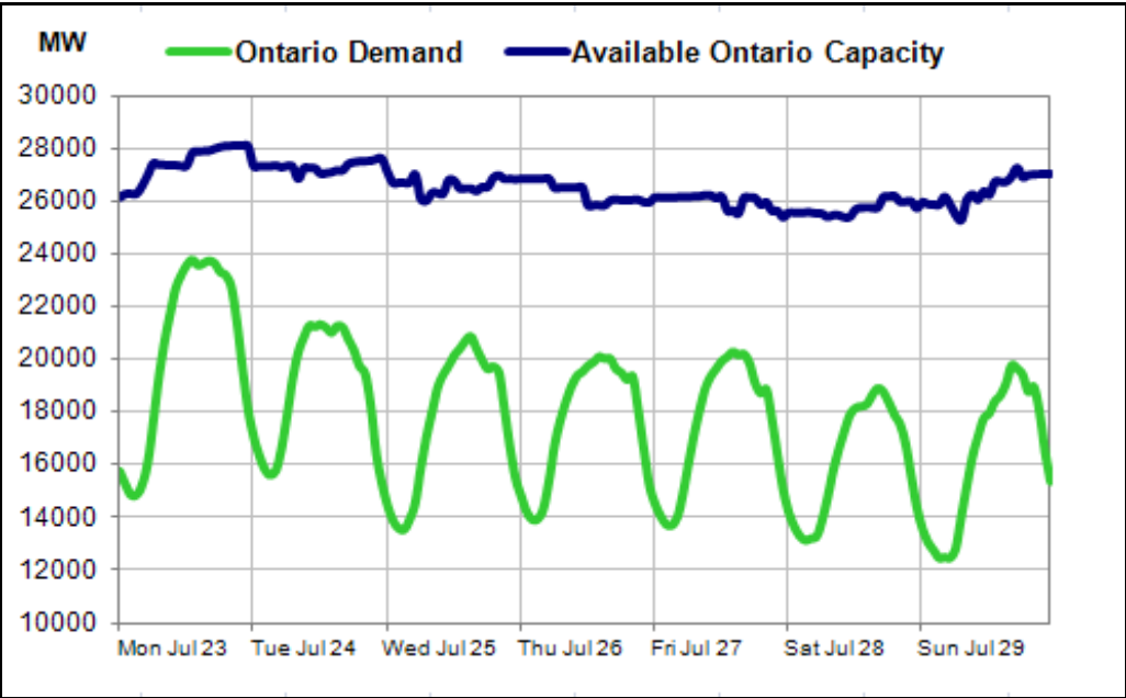
Hourly Ontario demand vs. available generation capacity within the province. Internal supply is supplemented by import capacity of up to 4,800 MW.
