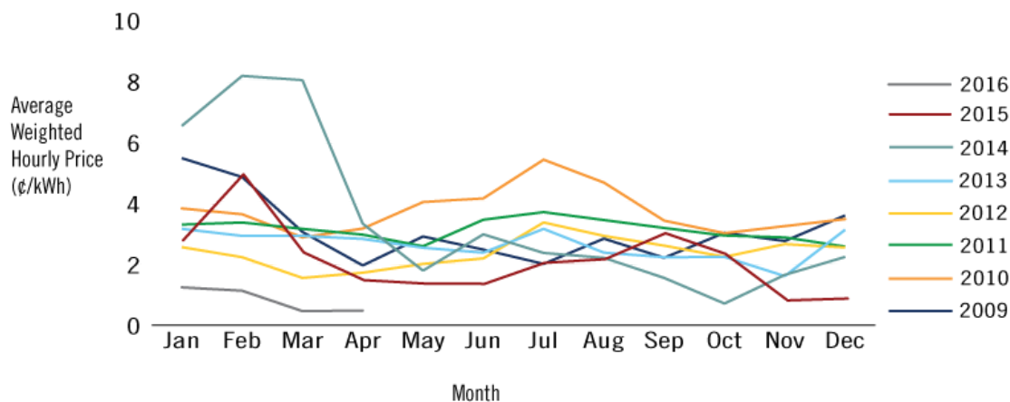
Average Weighted Hourly Price (¢/kWh)
